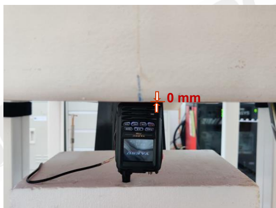
Photograph 7. Body, Bottom Edge, 0mm
