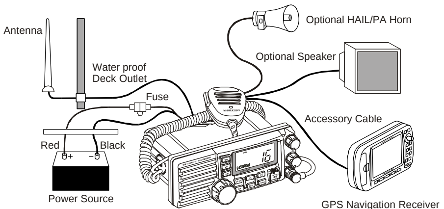
Figure 1. General Installation
