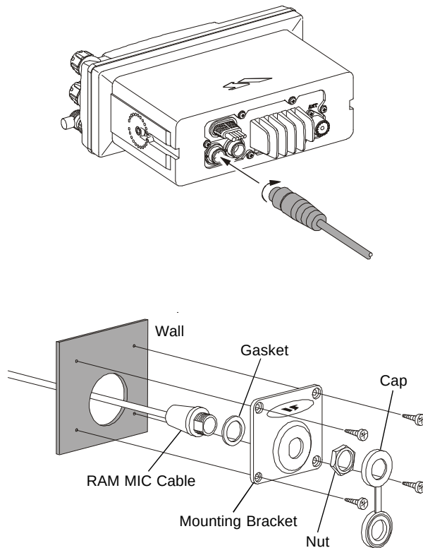
Figure 3. CMP25 RAM+ MIC Installation
