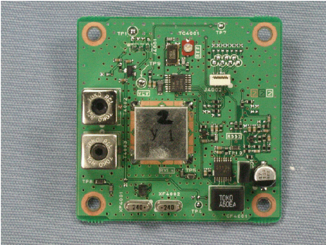
Side-A of SUB-RX-UNIT with shield case
