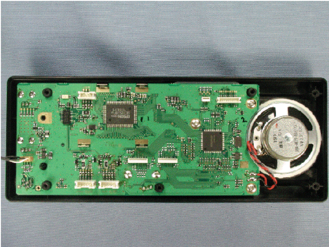
Inside of Panel with PWB
