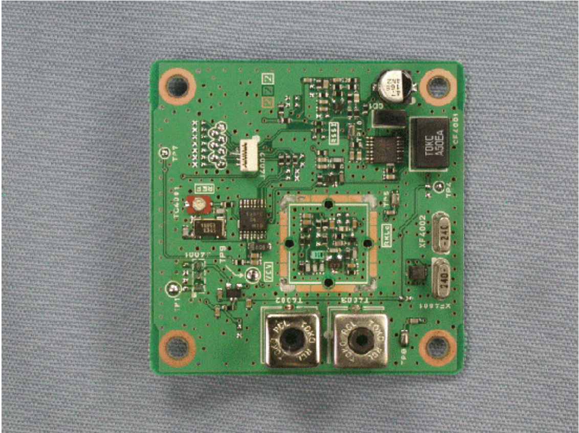
Side-A of SUB-RX-UNIT without shield case
