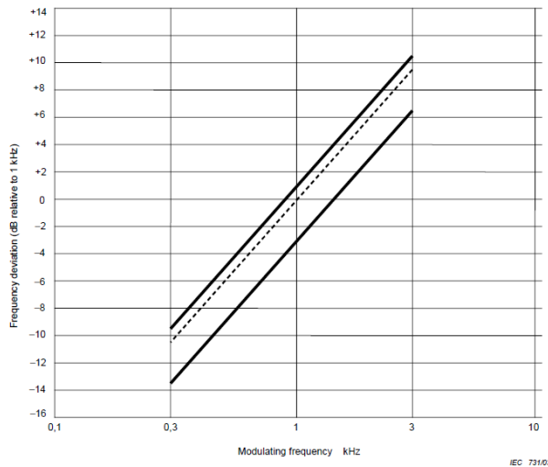
Figure 2 – Audiofrequency response
