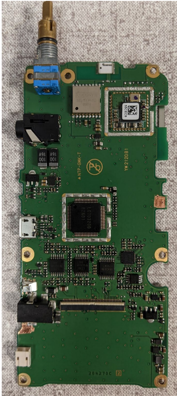
PCB Front, with Shield removed
