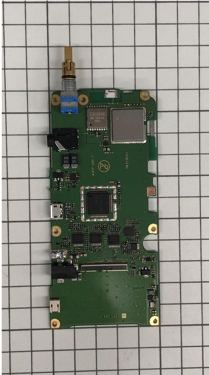
CNTL-UNIT
