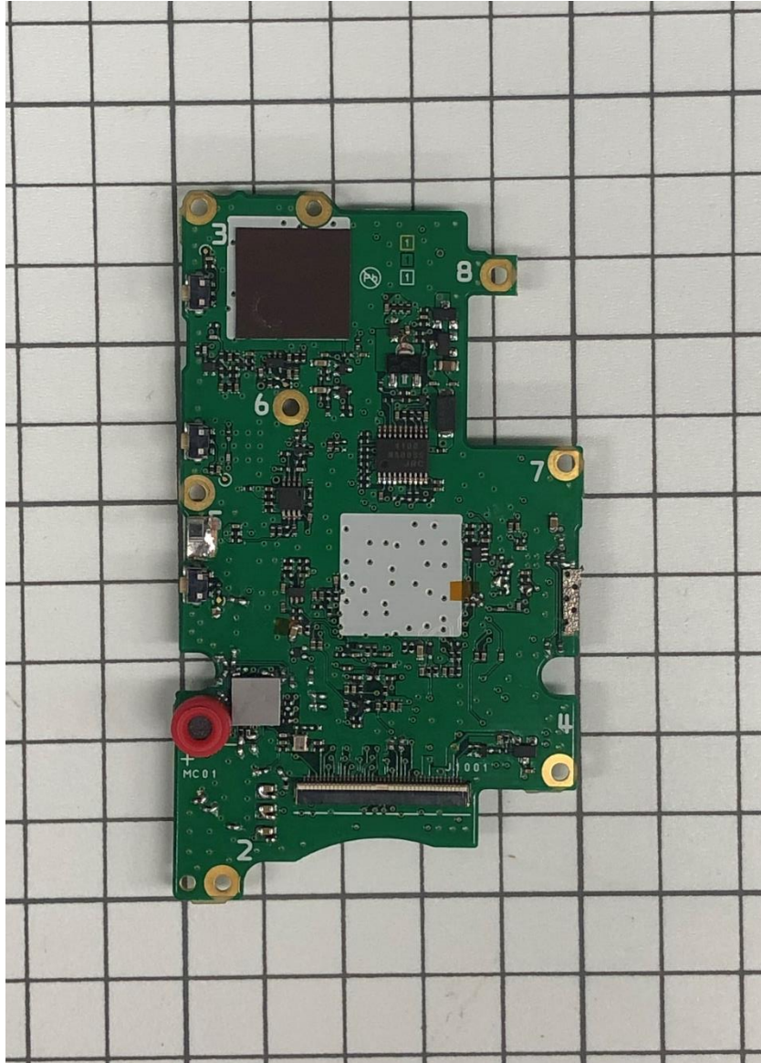
MAIN-UNIT
