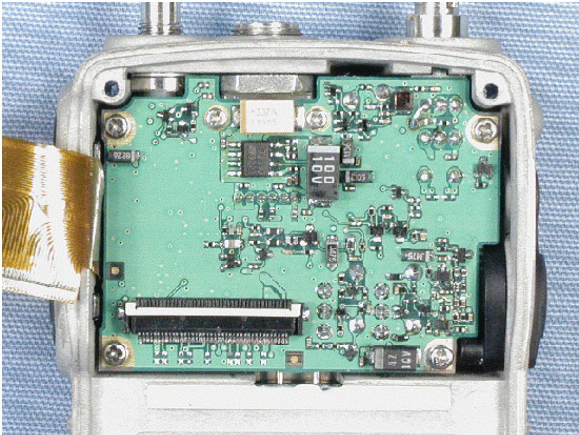
AF-UNIT in front case
