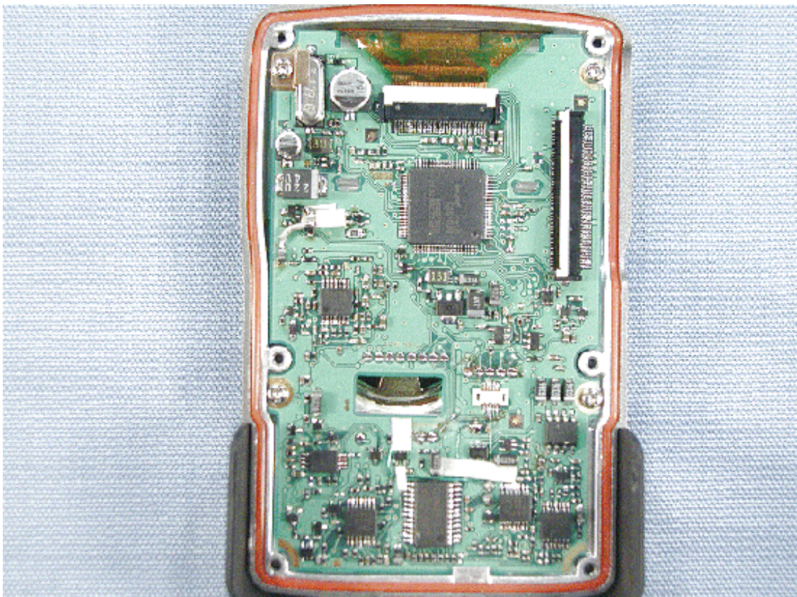
CNTL-UNIT in front case
