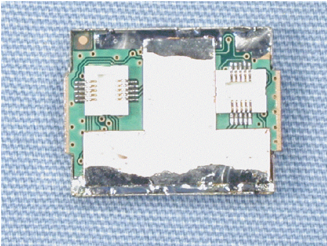
VCO-UNIT in shield case
