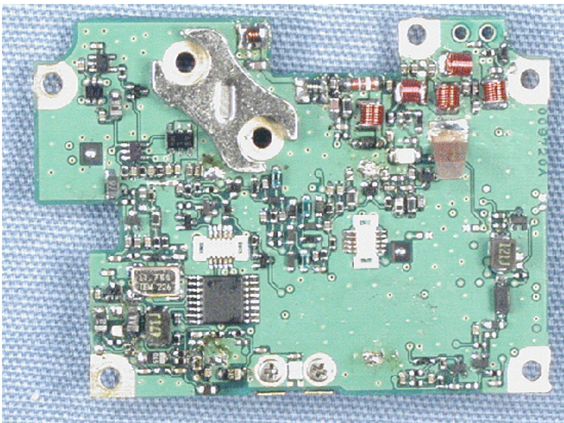
Side-B of RF-UNIT without VCO-UNIT
