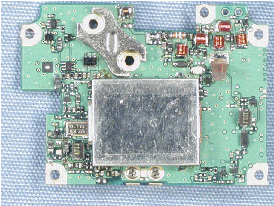
Side-B of RF-UNIT with VCO-UNIT
