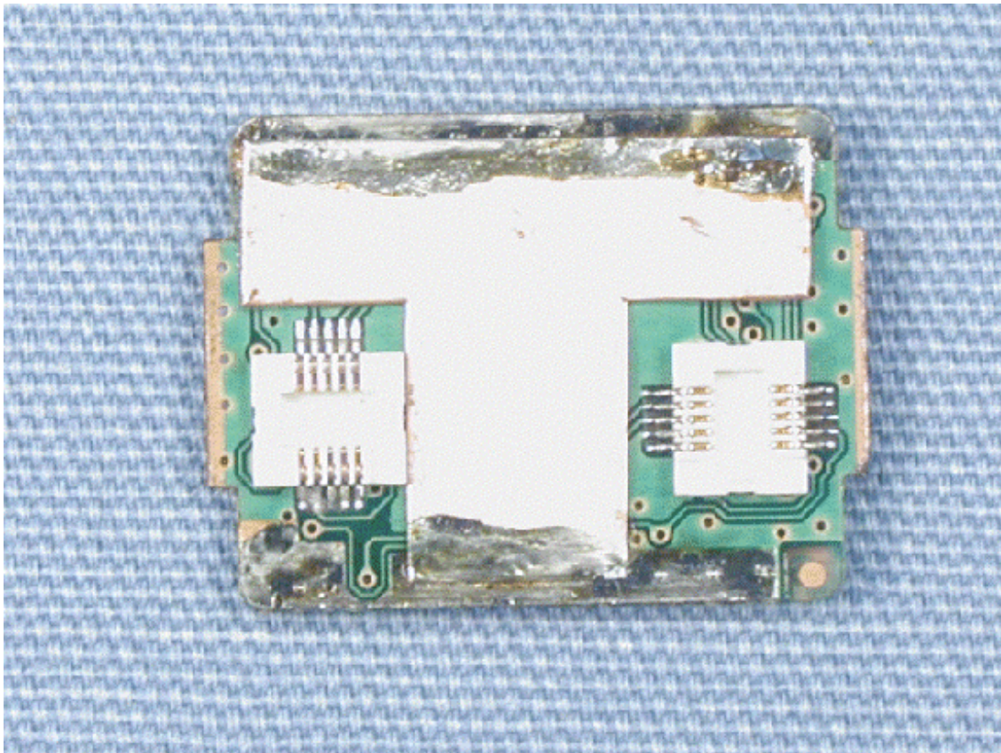
Side-B of VCO-UNIT
