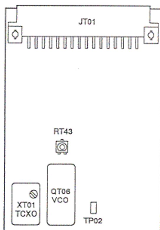
Figure 6-11 TX unit
