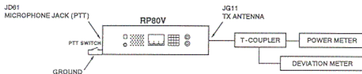
Figure 6-6 Tone deviation alignment
