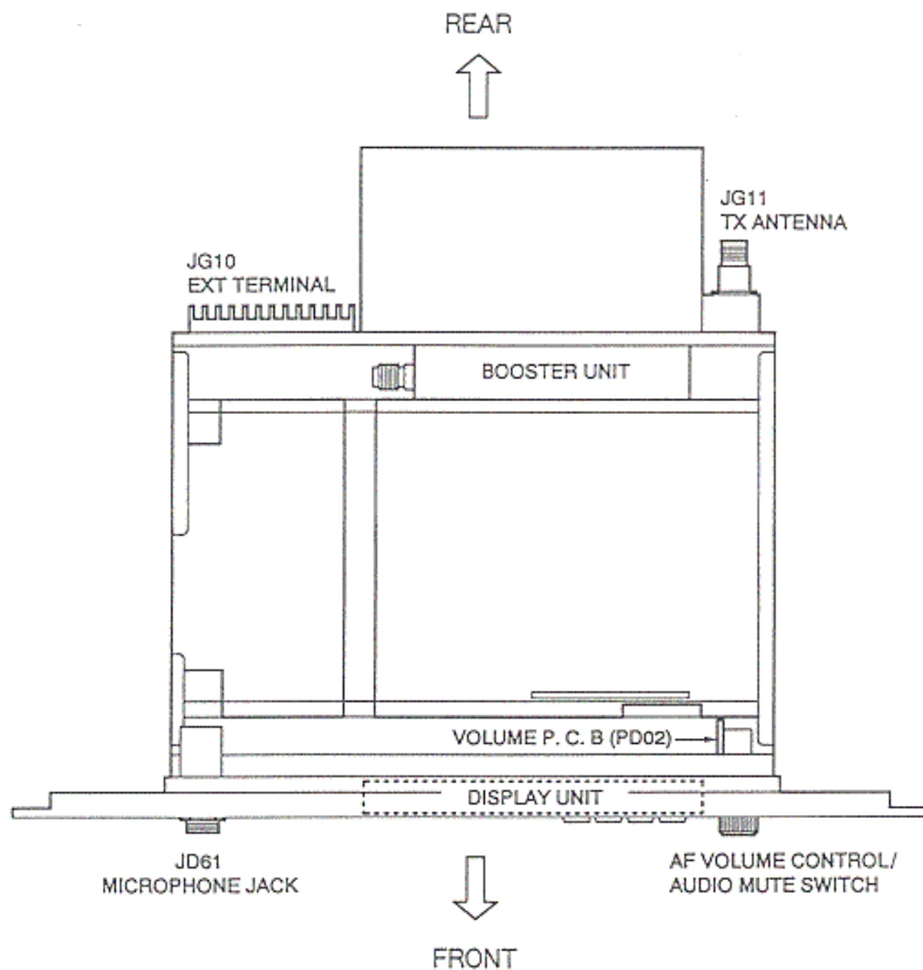
Figure 6-8 Top view
