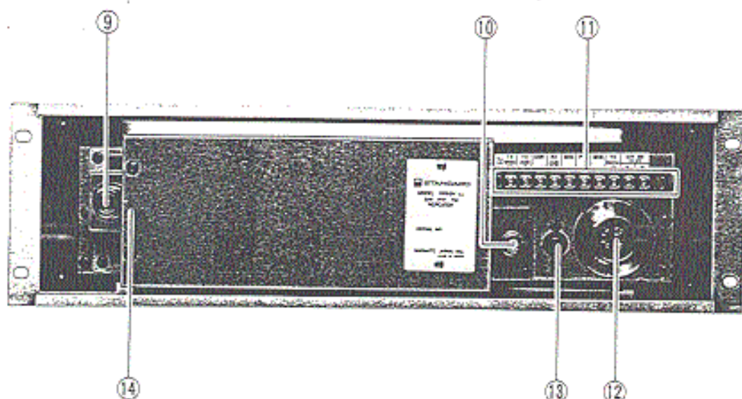
Figure 1-2 Rear Panel
