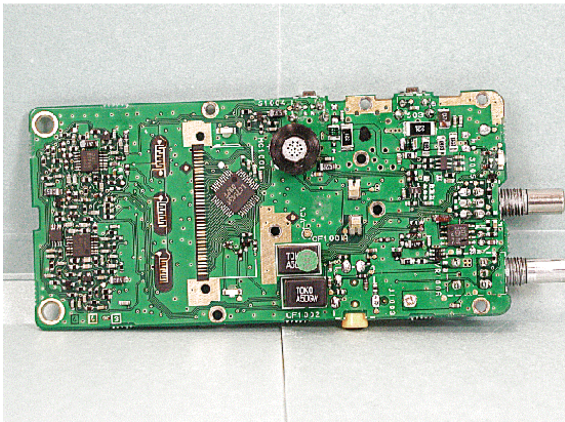
Side-A of PCB without LCD
