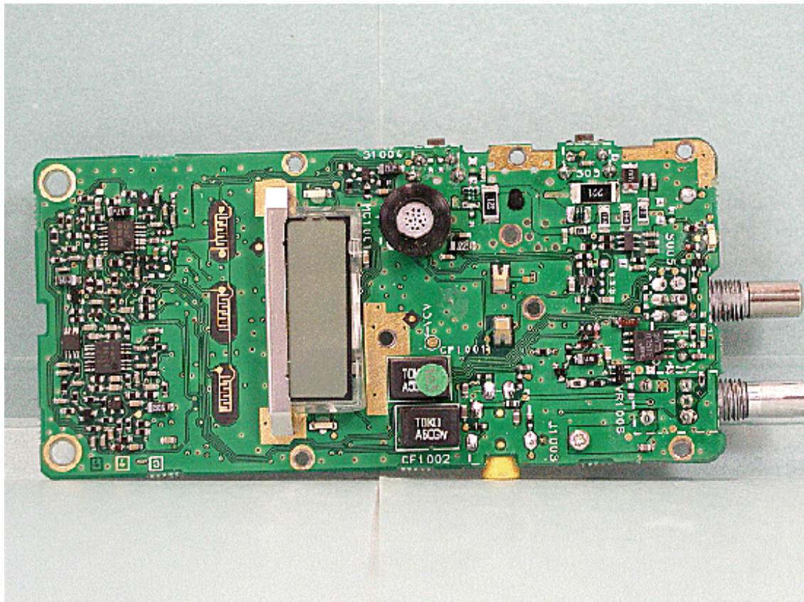
Side-A of PCB with LCD
