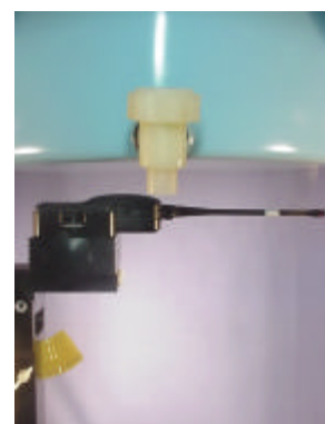
Face-Held SAR Test Setup
