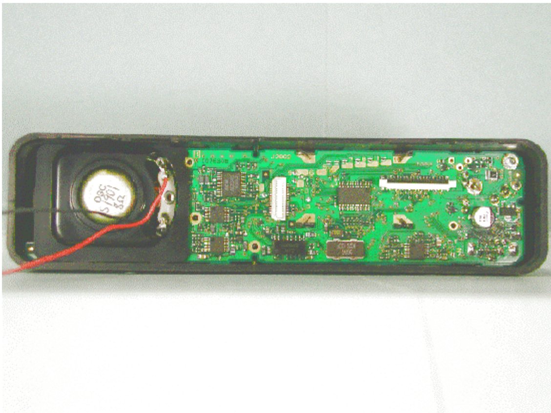
Inside front of panel with PWB
