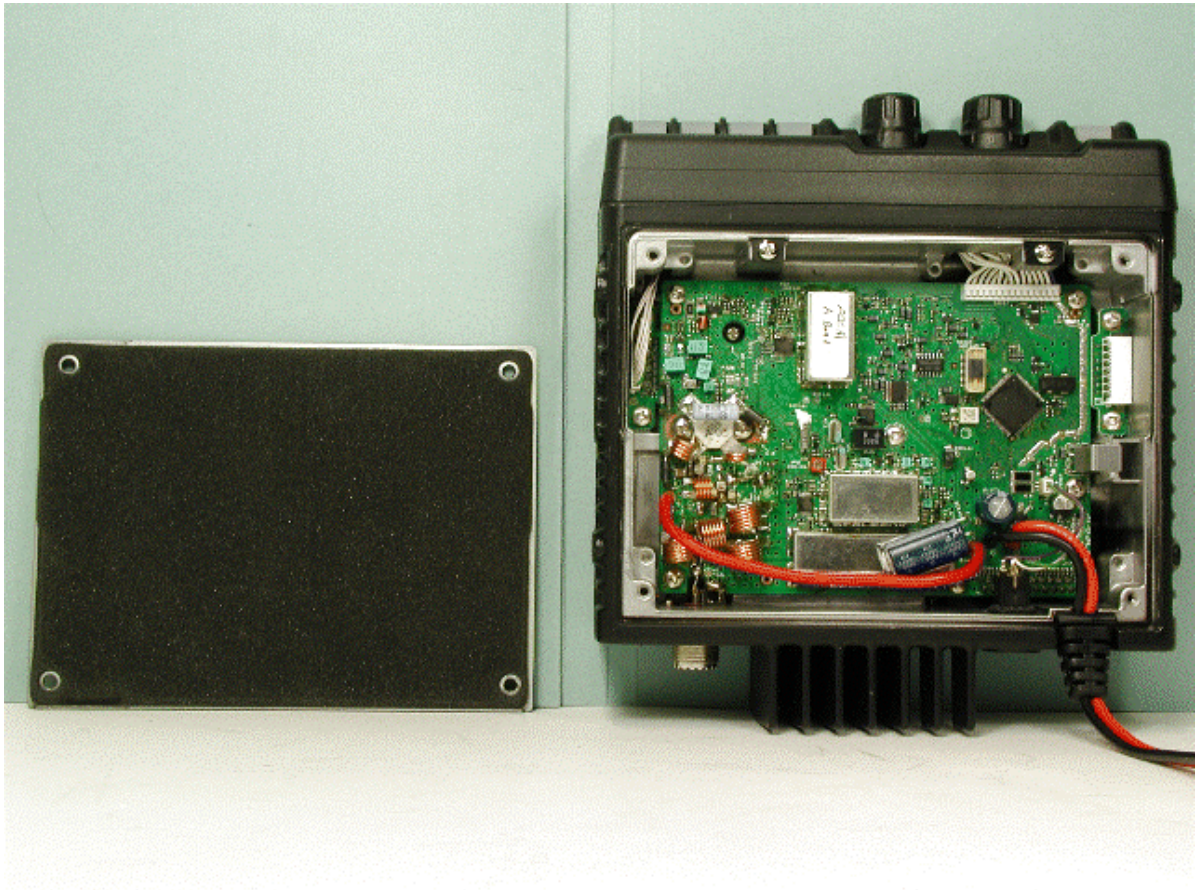
Top of EUT (Cover Opened)
