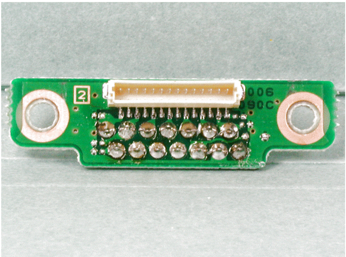
Solder Side of MIC-CONN-UNIT
