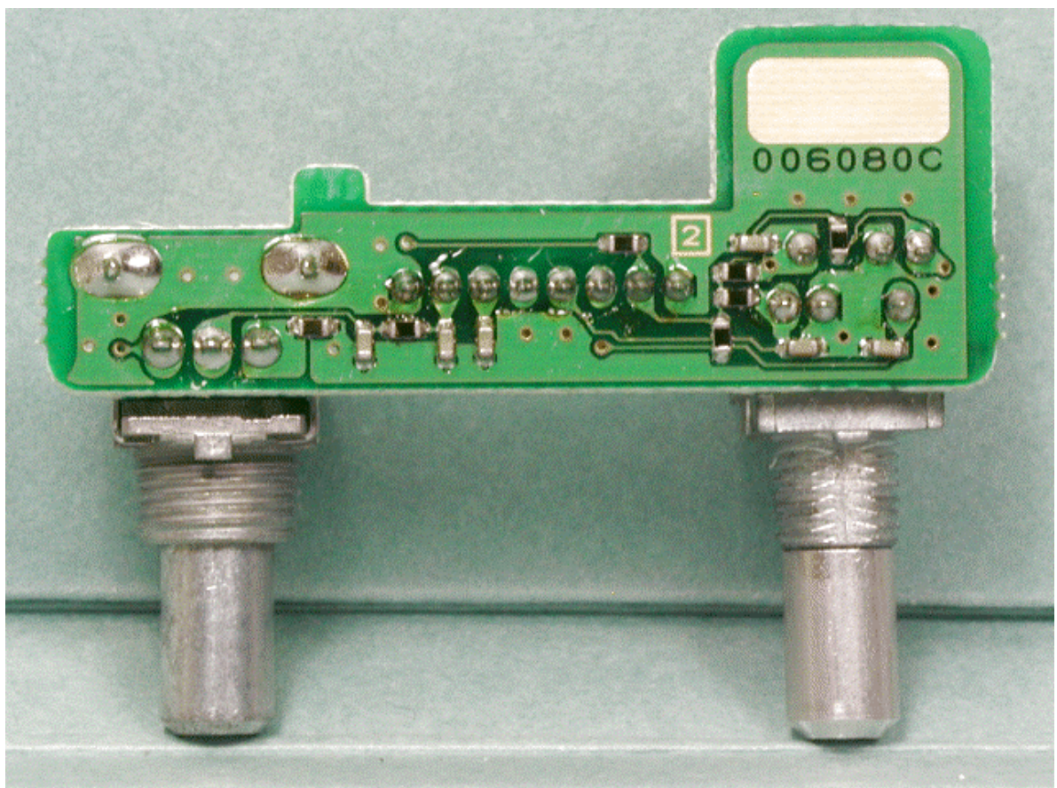
Solder Side of VR-UNIT
