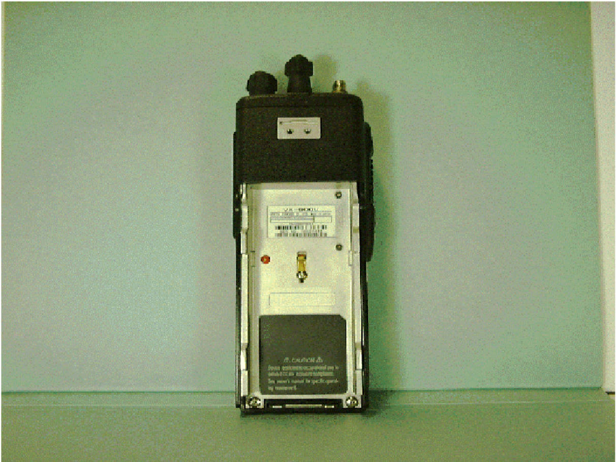
Back of EUT without Antenna
