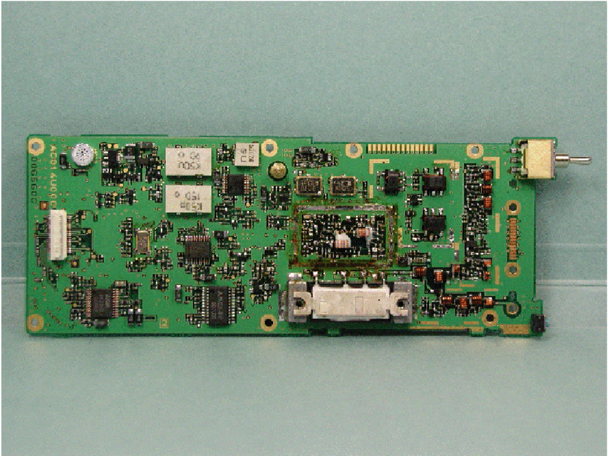
Bottom of PCB Board without VR/SW/Shield Case
