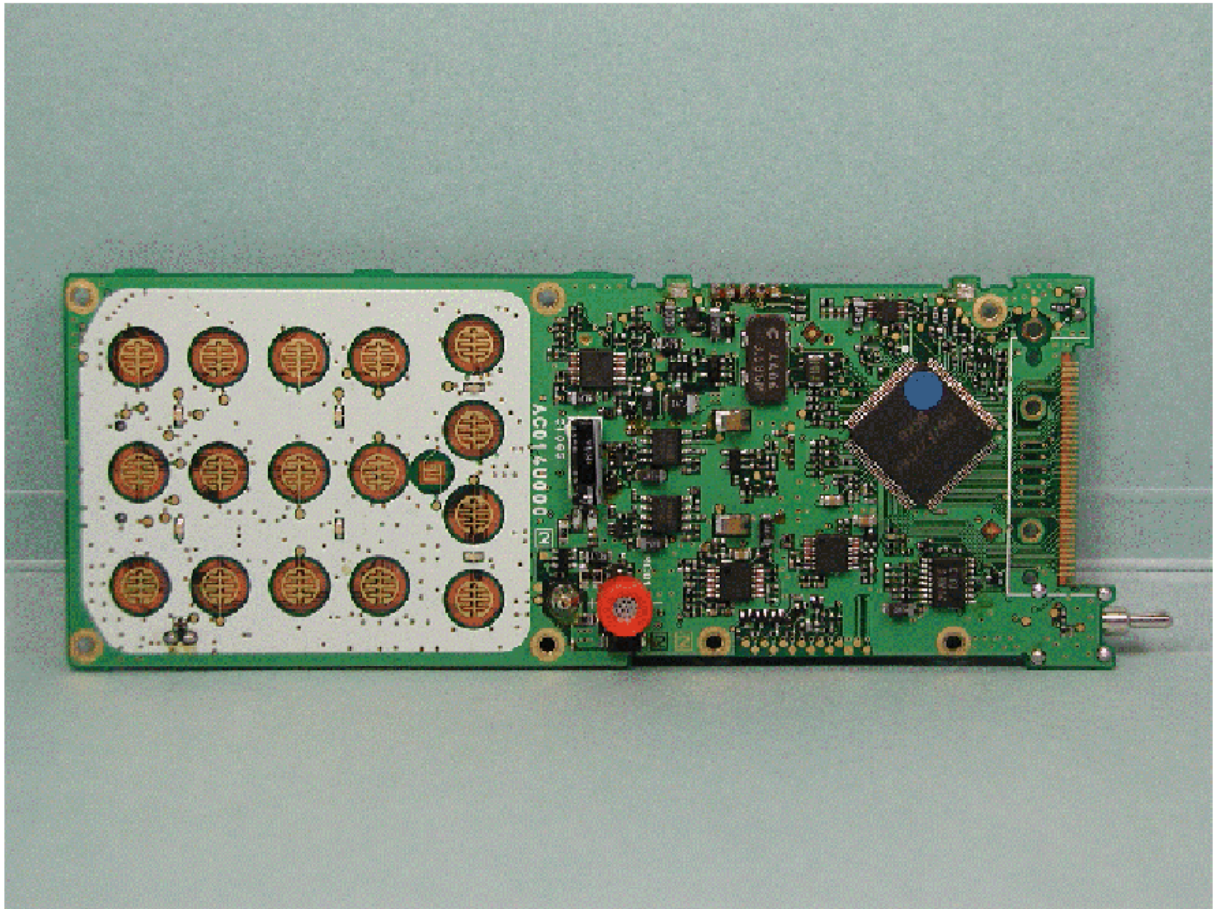
Top of PCB Board without VR/SW/Shield Case
