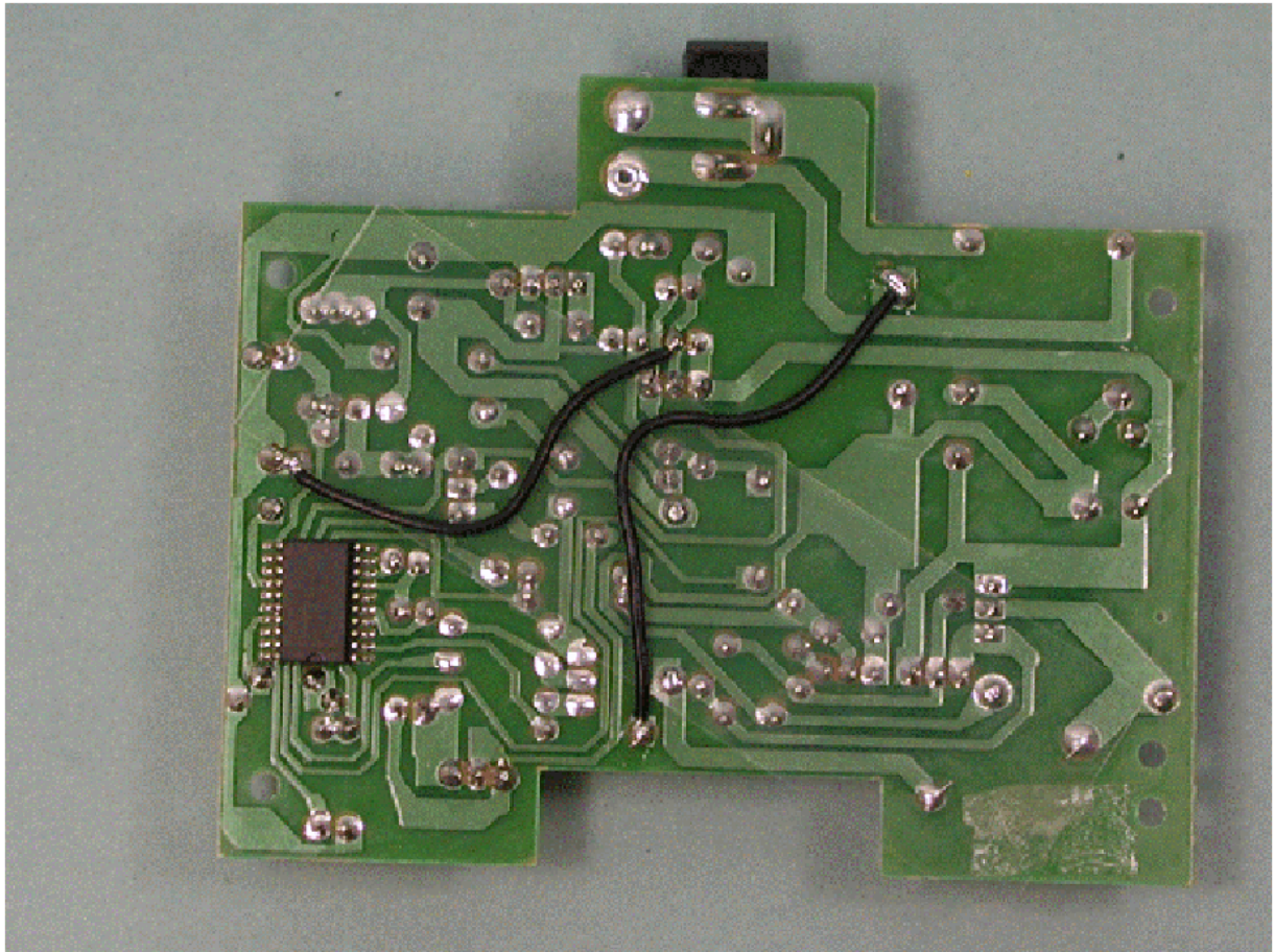
Solder Side of Battery Charger PCB
