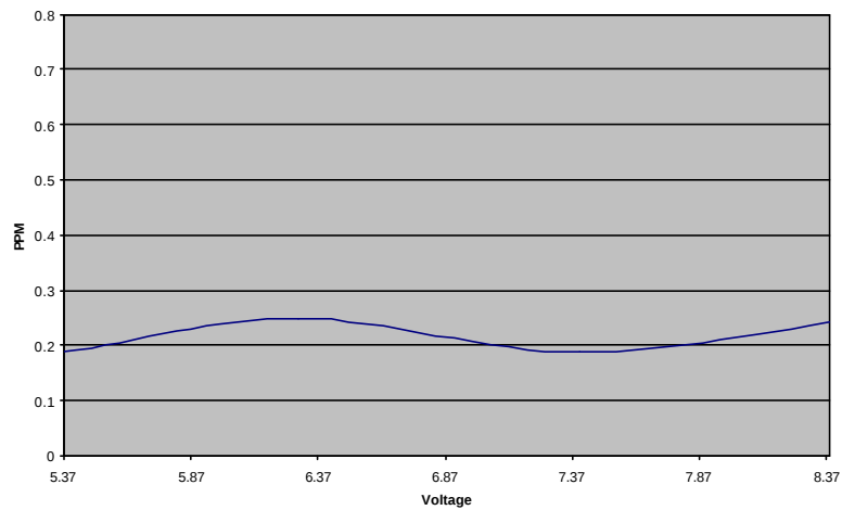
Voltage Frequency Stability (160.10MHz Narrowband)
