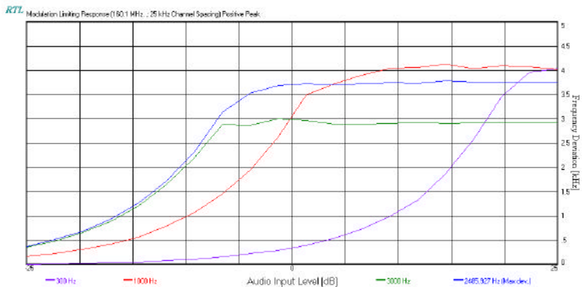
Channel 2 Wide Band Positive Peak
