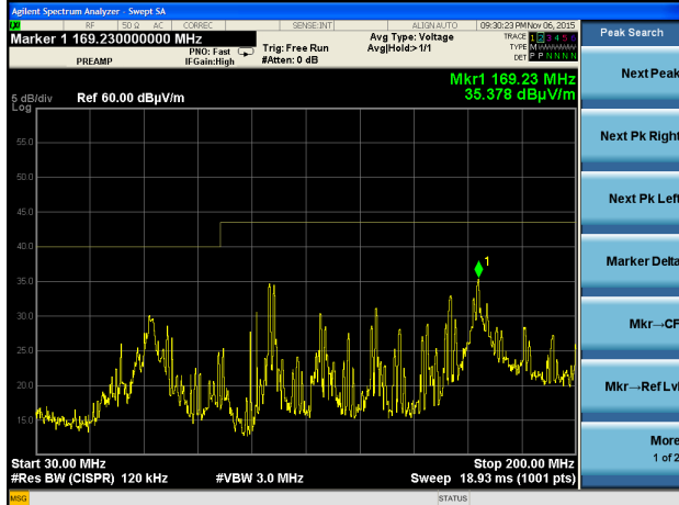
30-200 MHz Vertical
