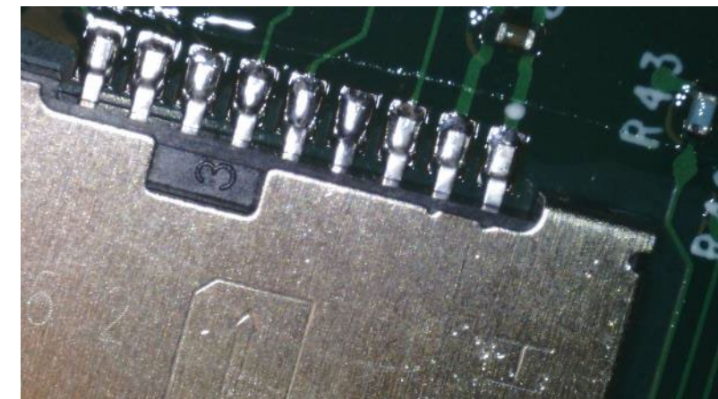
Close Up Photo of SIM Card Holders
