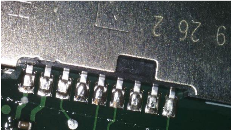
Close Up Photo of SIM Card Holders
