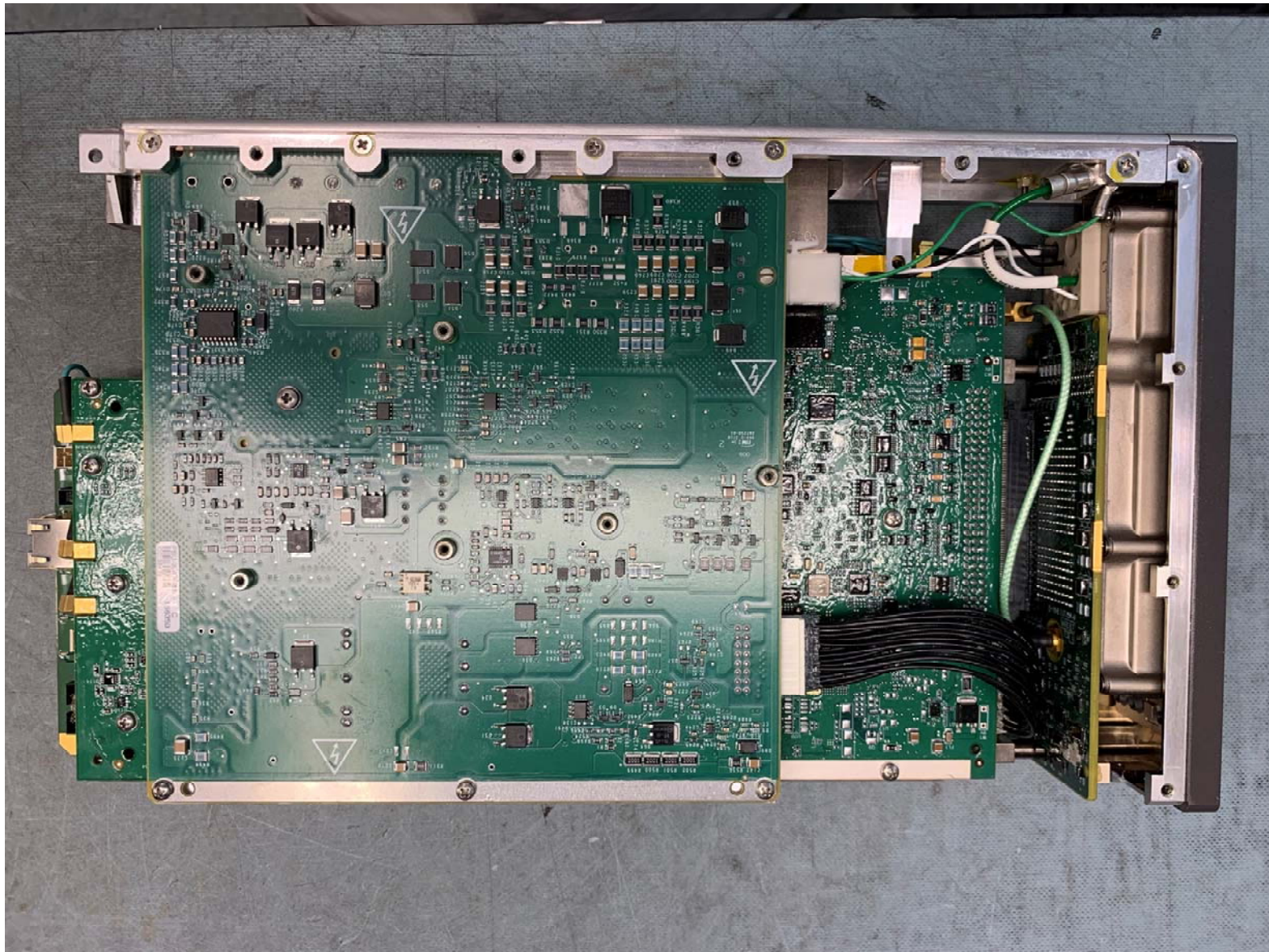
Figure 10: 90402651-000 Aspire 400 SDU Internal View Rear Interconnect
