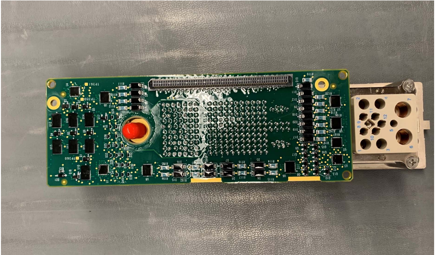
Figure 6: PBC-90404045 Backplane Card Bottom View
