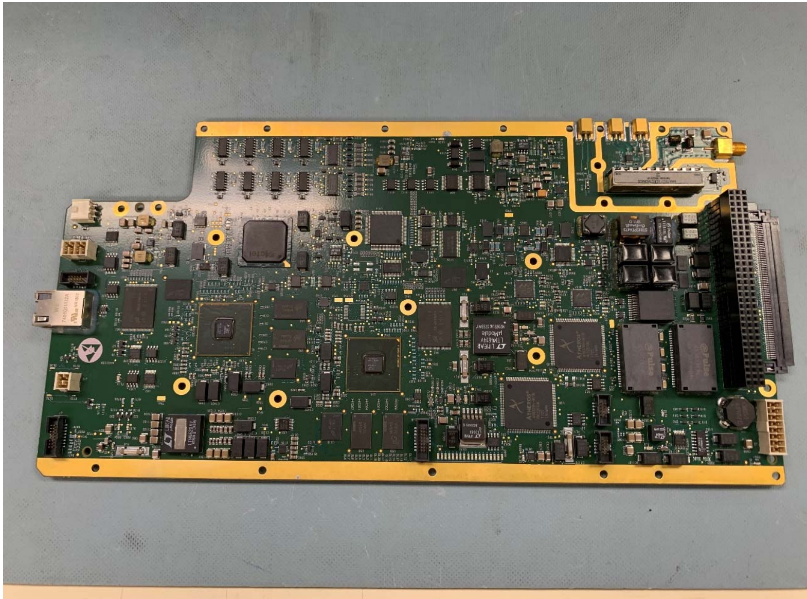
Figure 3: PBC-90404046 MPC Top View Without Heat Sink
