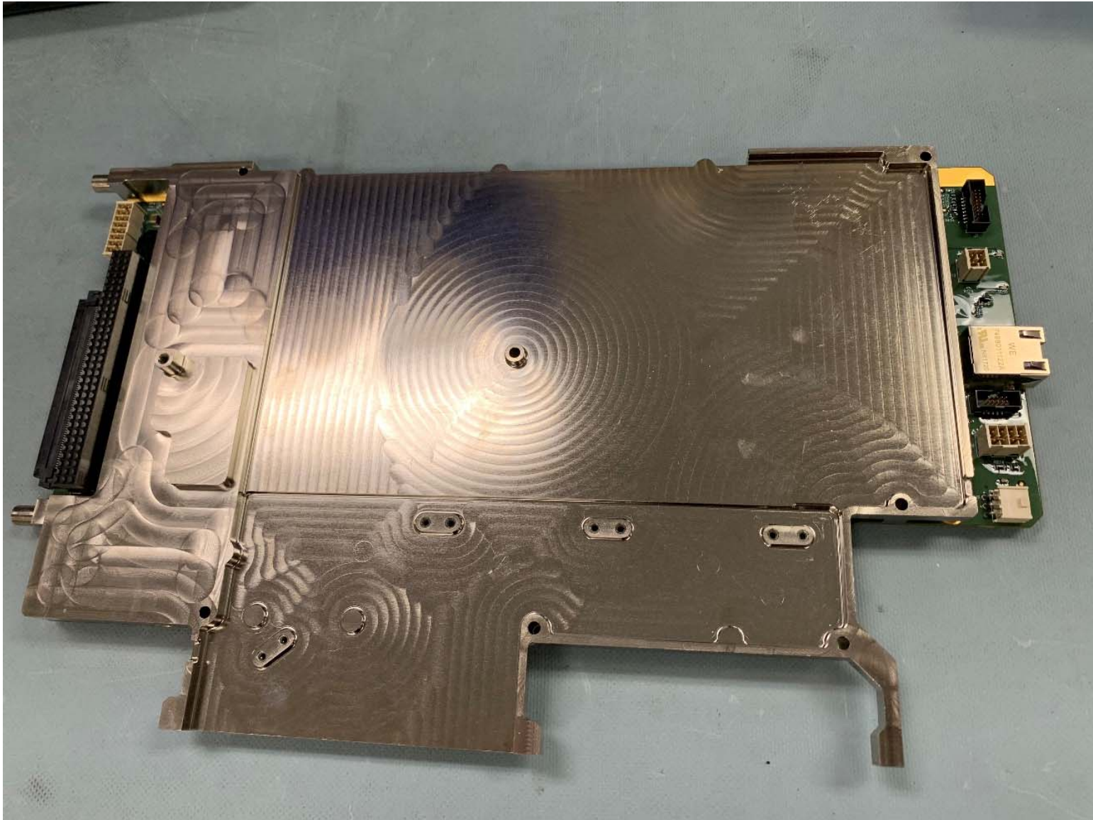
Figure 2: PBC-90404046 MPC Top View with Heat Sink
