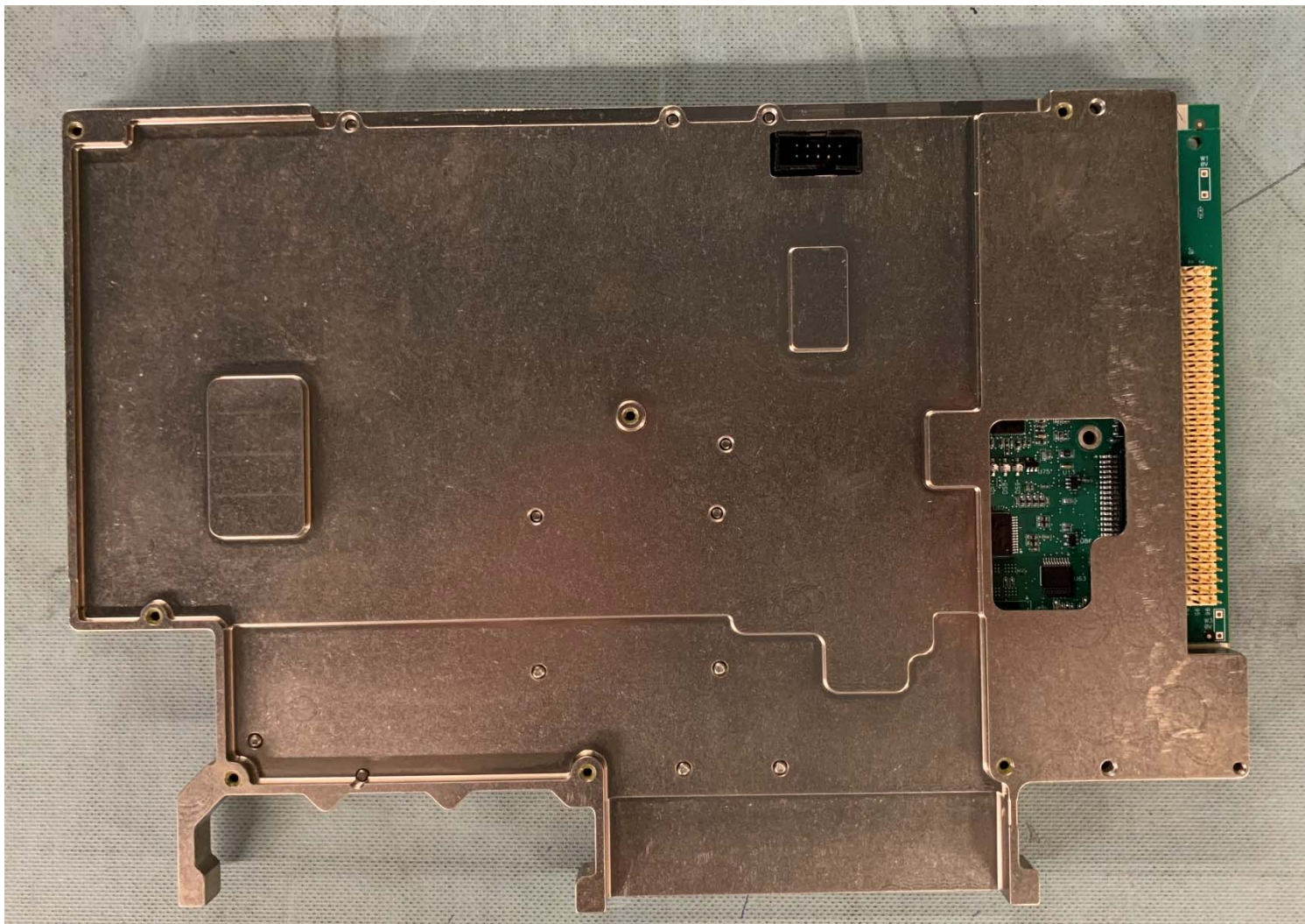
Figure 9: PBC-90600207 DABC Top View with Heat Sink
