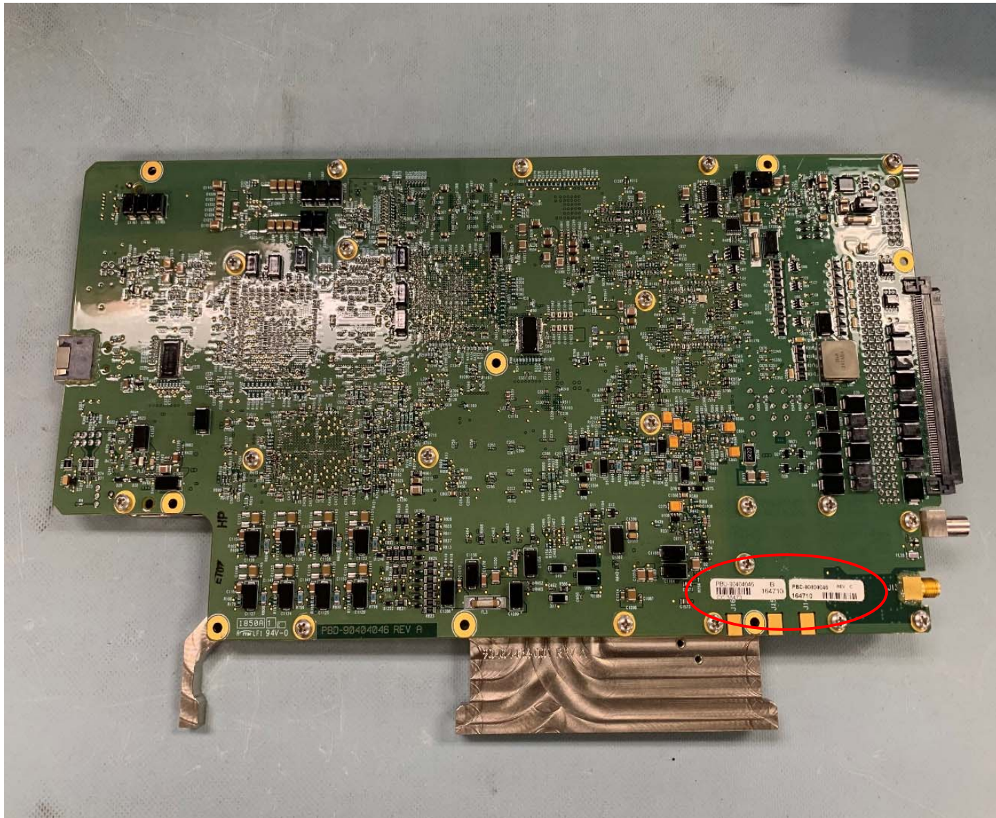
Figure 1: PBC-90404046 MPC Bottom View with Heat Sink
