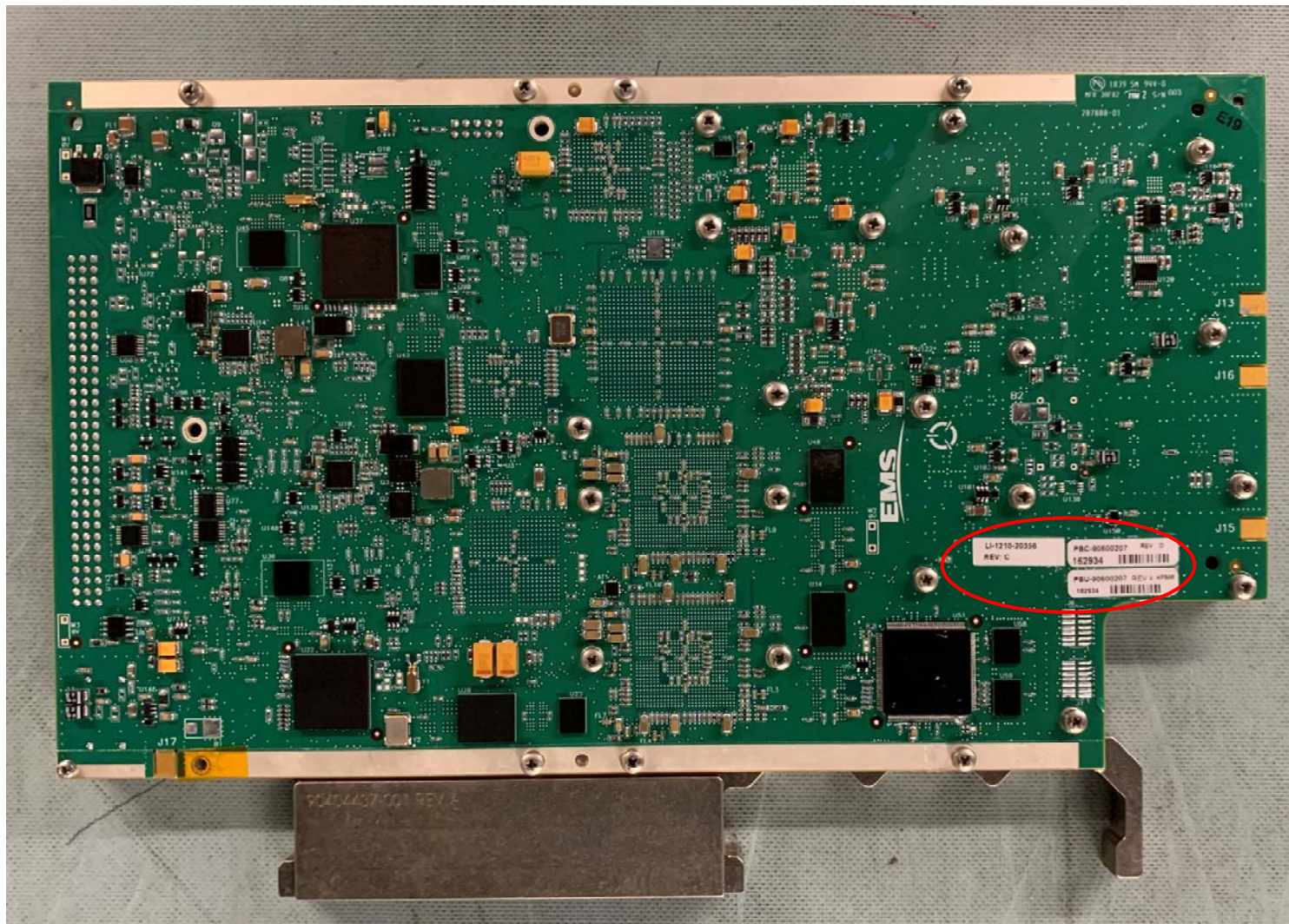
Figure 8: PBC-90600207 DABC Bottom View with Heat Sink
