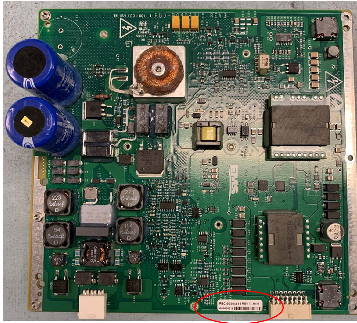
Figure 4: PBC-90404415 AC Power Supply Top View
