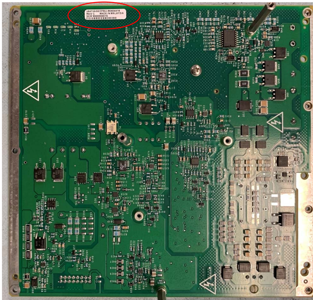
Figure 5: PBC-90404415 AC Power Supply Bottom View
