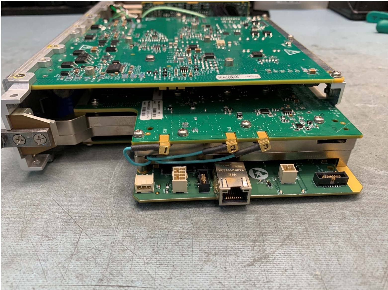
Figure 11: 90402651-000 Aspire 400 SDU Internal View Front Interconnect
