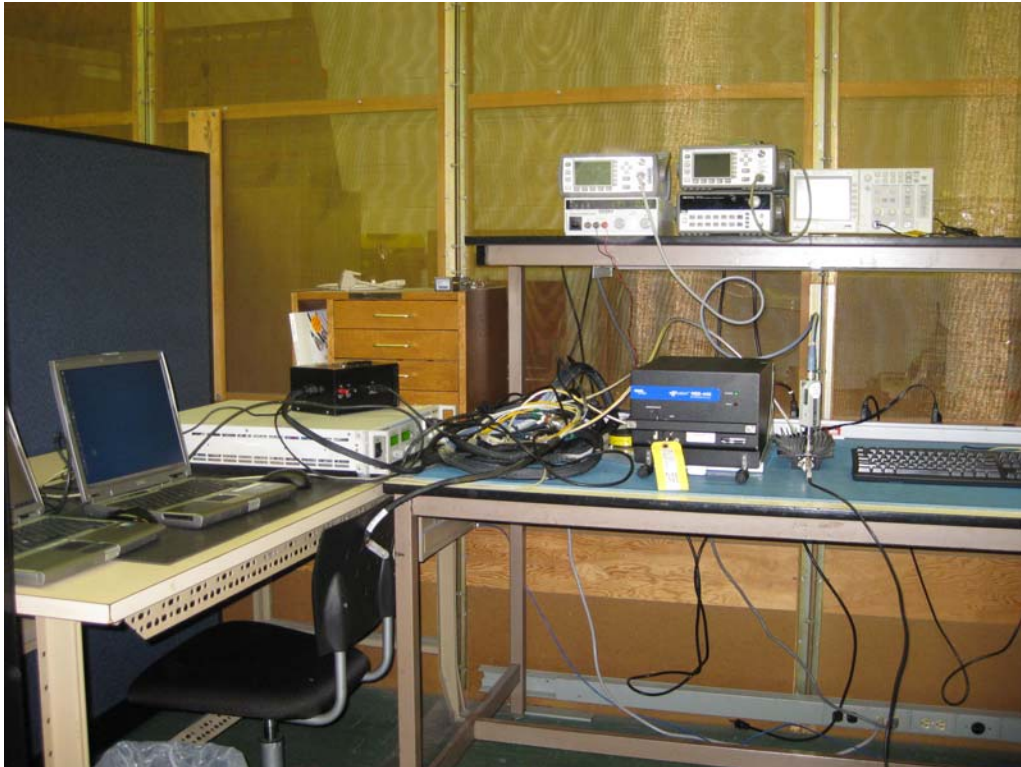
Conducted
