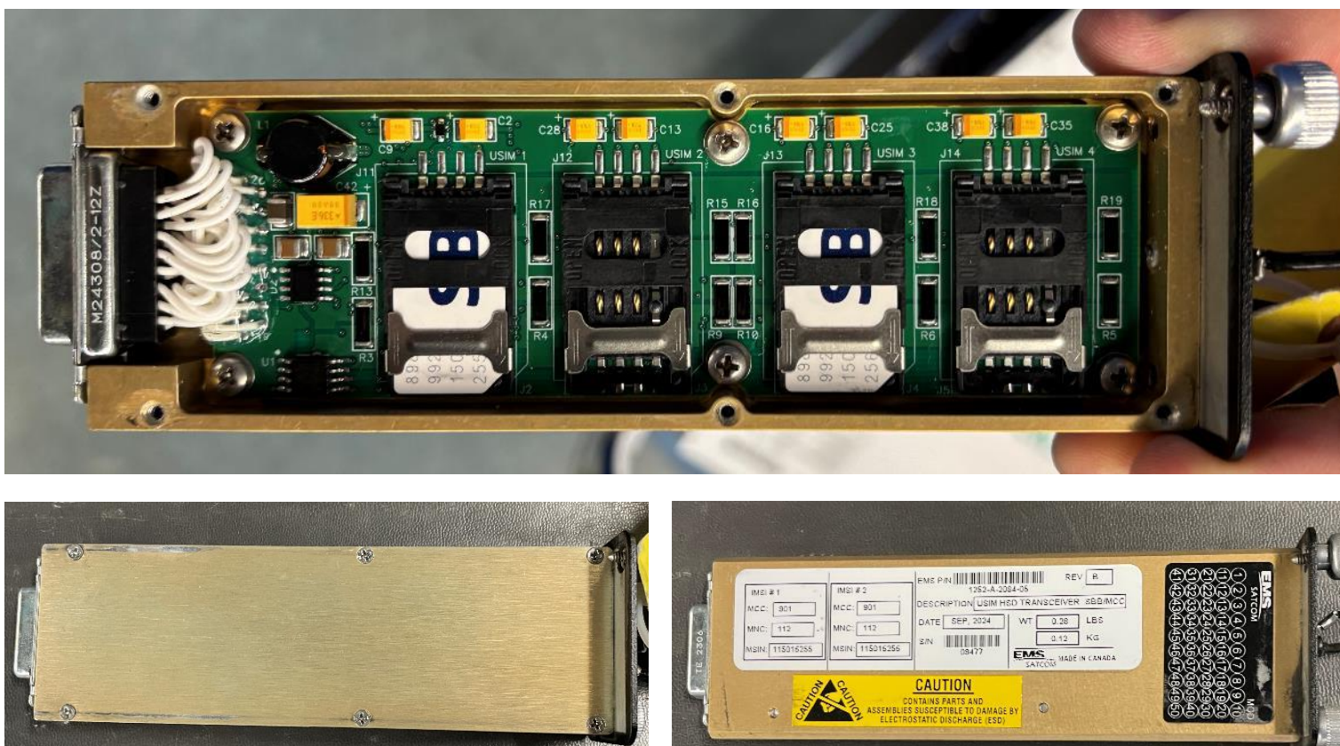
Figure 1: 1252-A-2084 HSD XCEIVER
