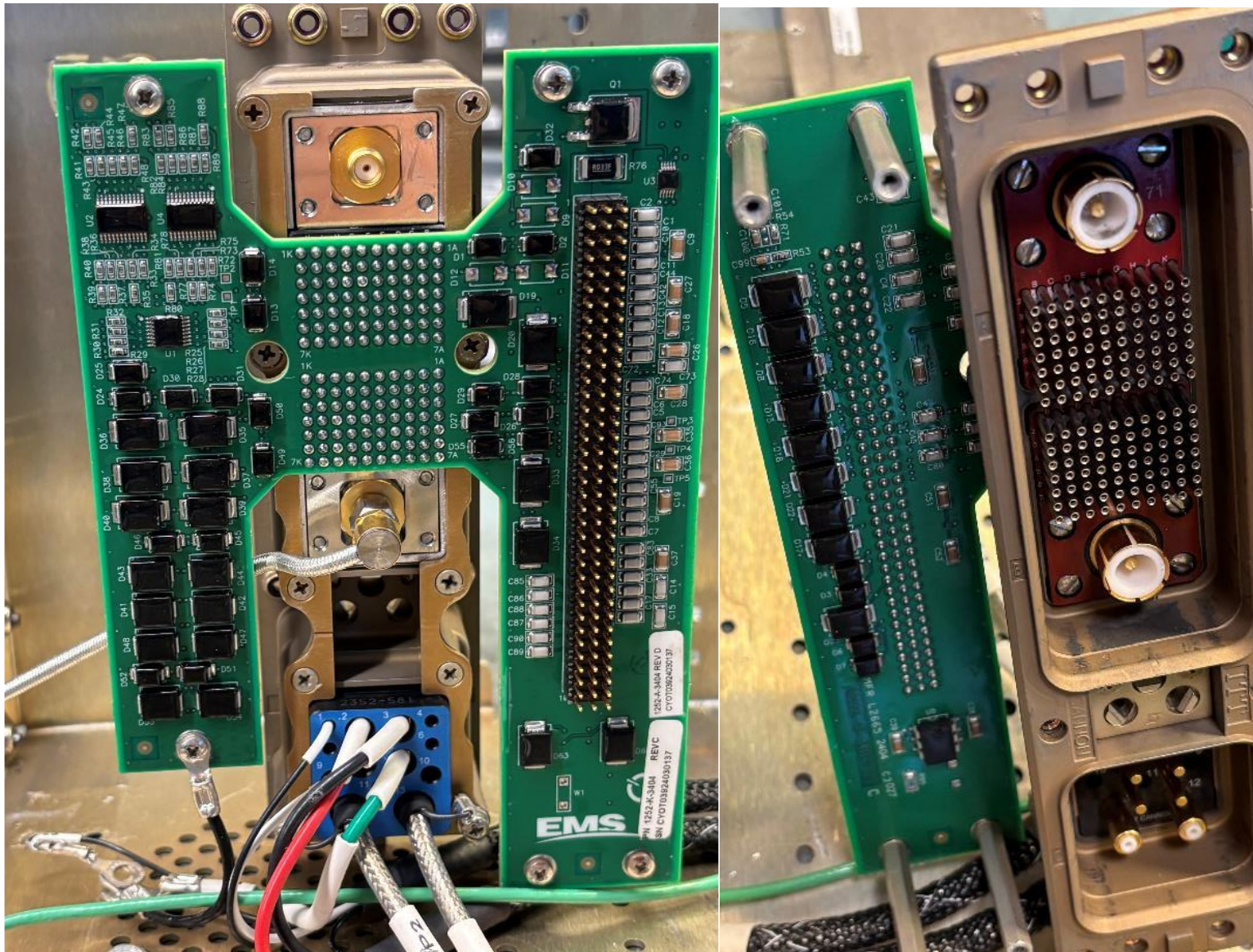
Figure 5: 1252-K-3404 CCA Motherboard
