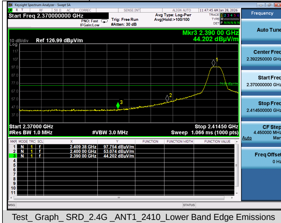
Test Graph for Average Measurement- Horizontal
