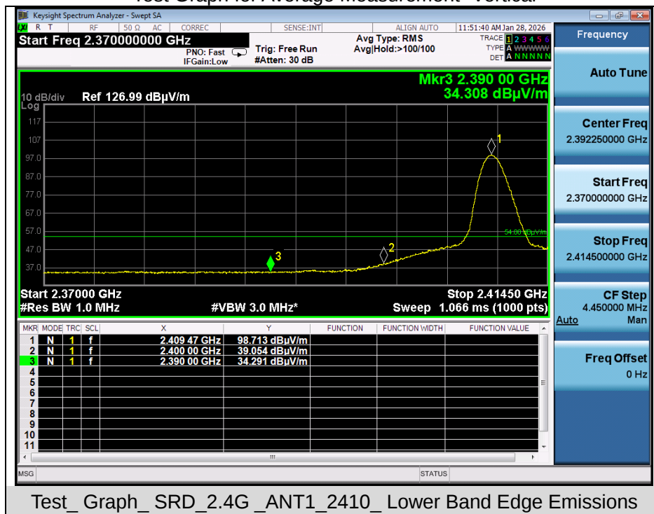
Test Graph for Average Measurement- Vertical
