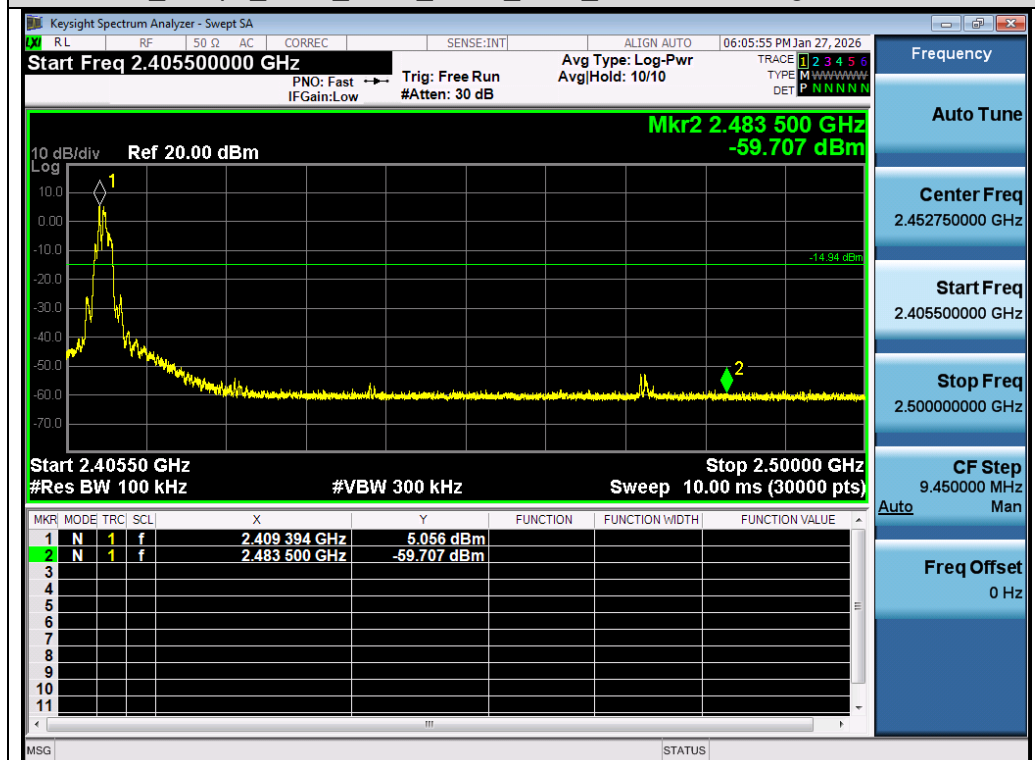
Test_Graph_SRD_2.4G_ANT1_2410_Higher Band Edge Emissions
