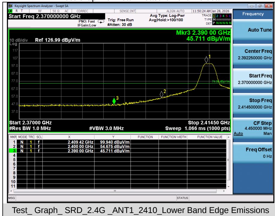
Test Graph for Peak Measurement- Vertical
