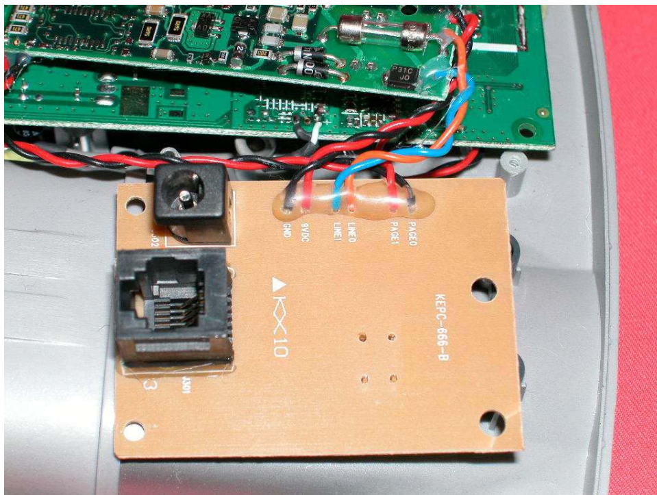
Base Telephone Jack, Adaptor Jack, and Page key PCB front side
