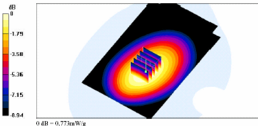
SAR Test Result for GMRS Face SAR -1.5 cm Spacing-Channel 15
