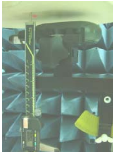
Figure 11.1 SAR Test Setup -----Face Position-----
