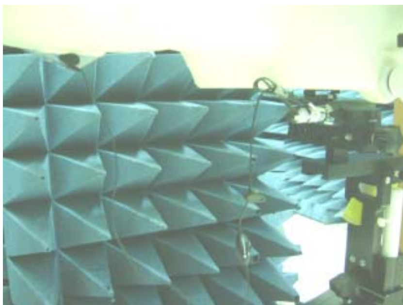
Figure 11.4 Body SAR Test Setup -----w / Belt Clip-----
