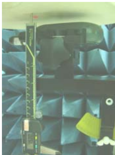
Figure 11.2 SAR Test Setup -----Face Position-----
