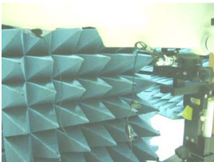
Figure 11.3 SAR Test Setup -----w / Belt Clip-----
