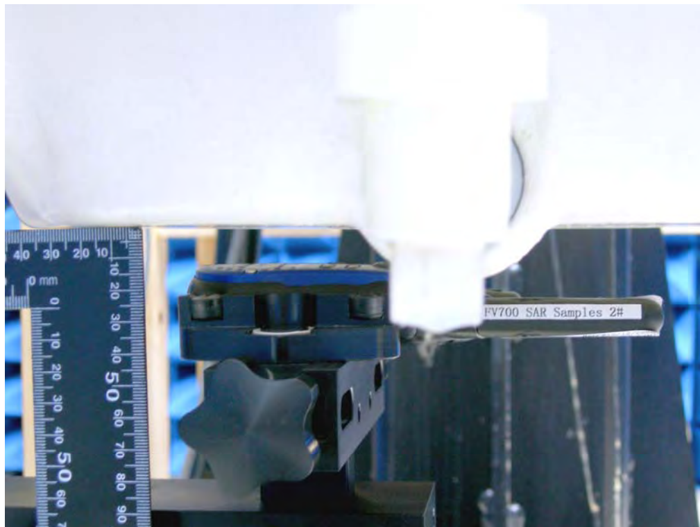
Figure 17. SAR Test Setup Face Position
