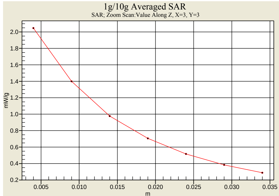
Head-Tissue-Simulating-Liquid 450MHz _2006.12.21
