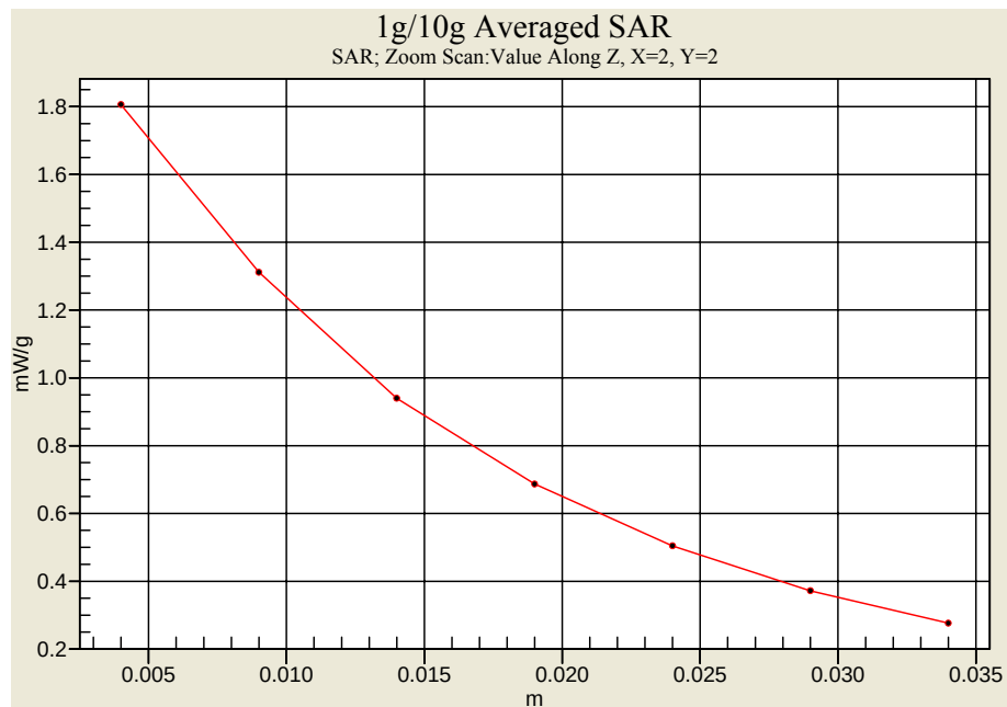
GMRS Body SAR w/o Belt-clip -1.5 cm Spacing _ CH15 NI-MH
