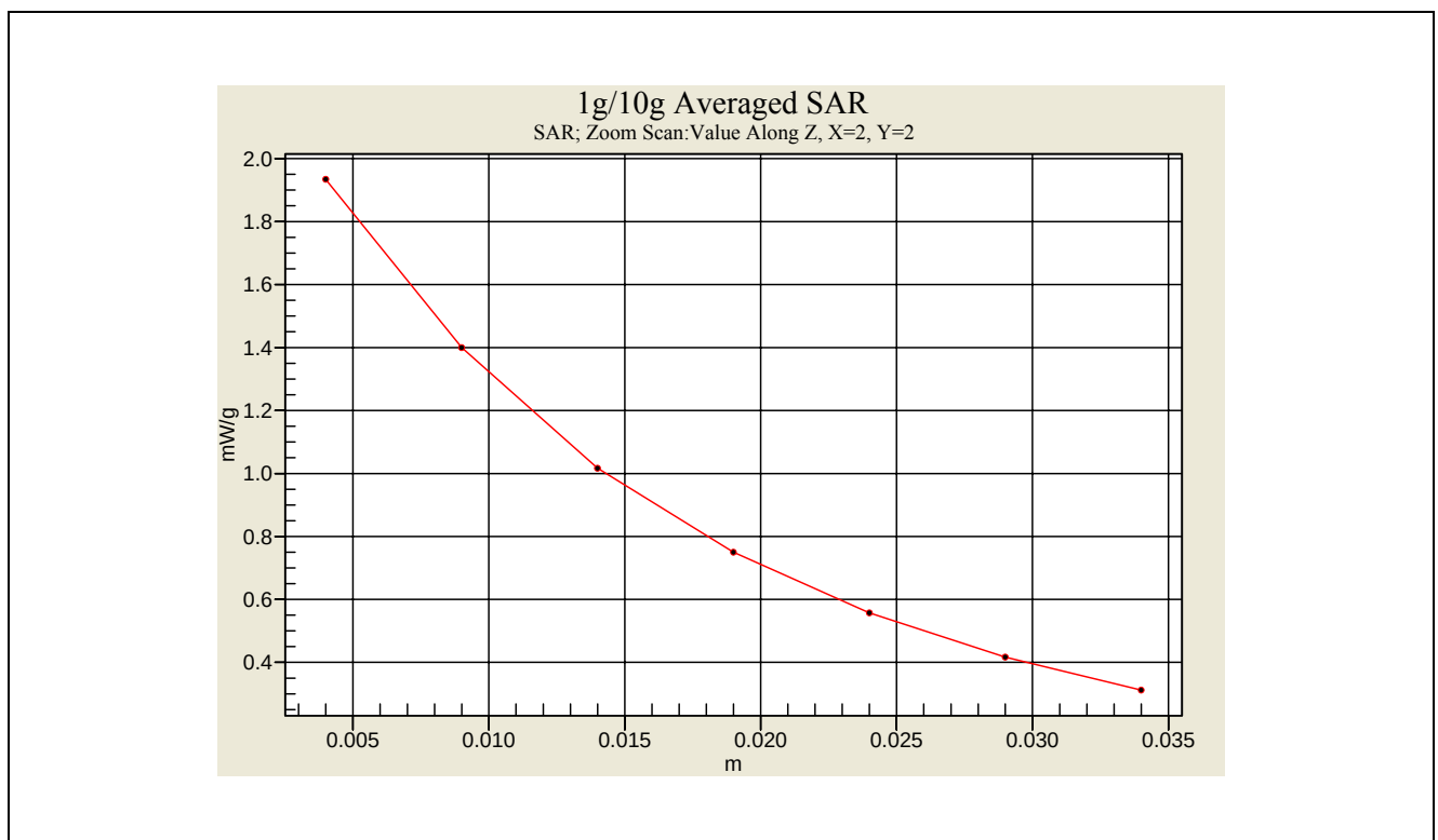
GMRS Face SAR -1.5 cm Spacing _ CH4 NI-MH
