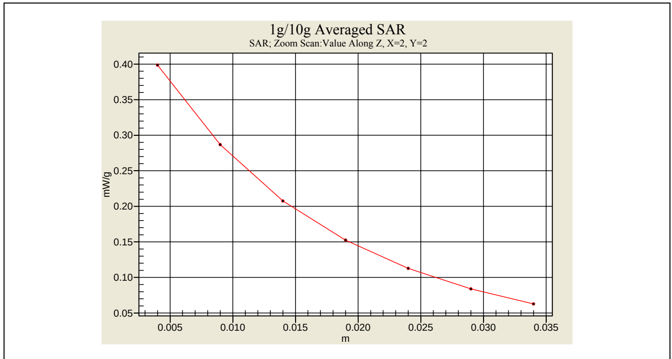
FRS Face SAR -1.5 cm Spacing _ CH14 NI-MH
