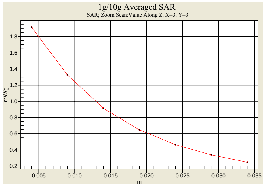
Body-Tissue-Simulating-Liquid 450MHz _2006.12.21
