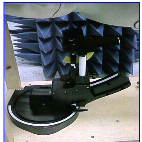
Figure 12. Device Holder
