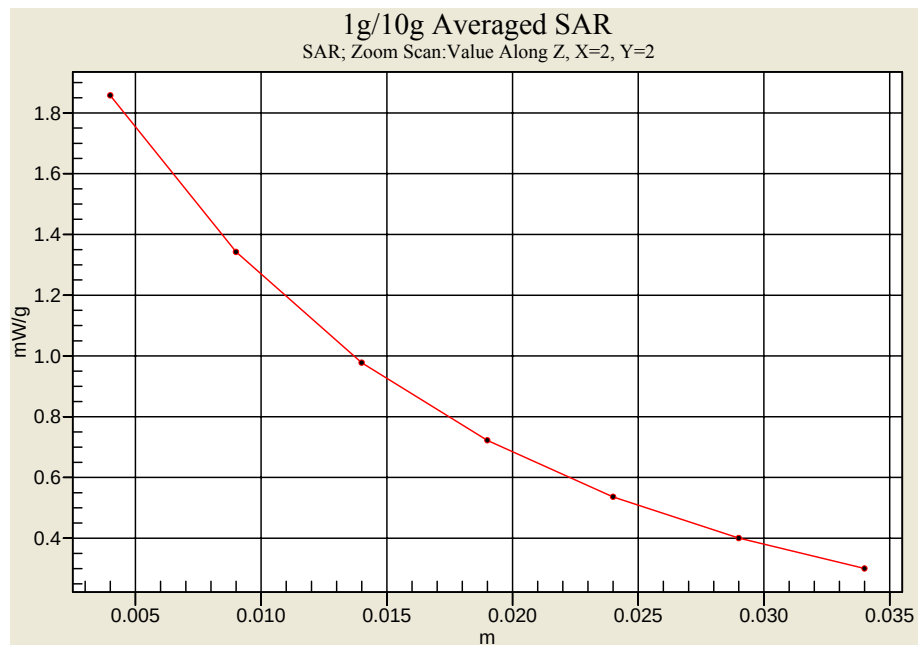
GMRS Body SAR with Belt-clip _ CH15 NI-MH
