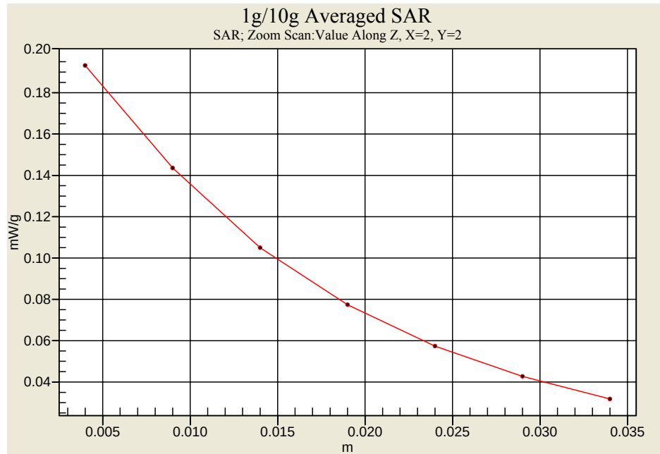
FRS Body SAR with Belt-clip _ CH11 NI-MH
