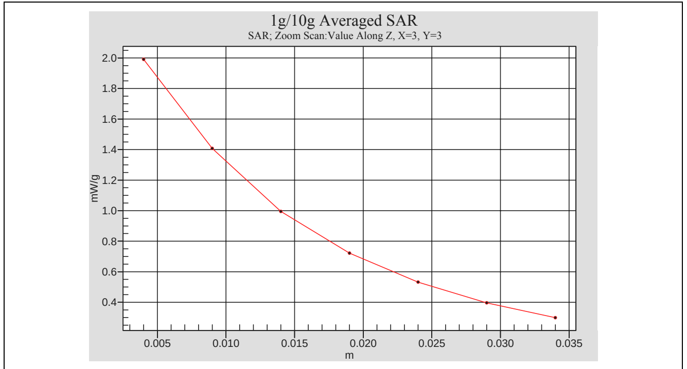
Body-Tissue-Simulating-Liquid 450MHz_2007.01.08
