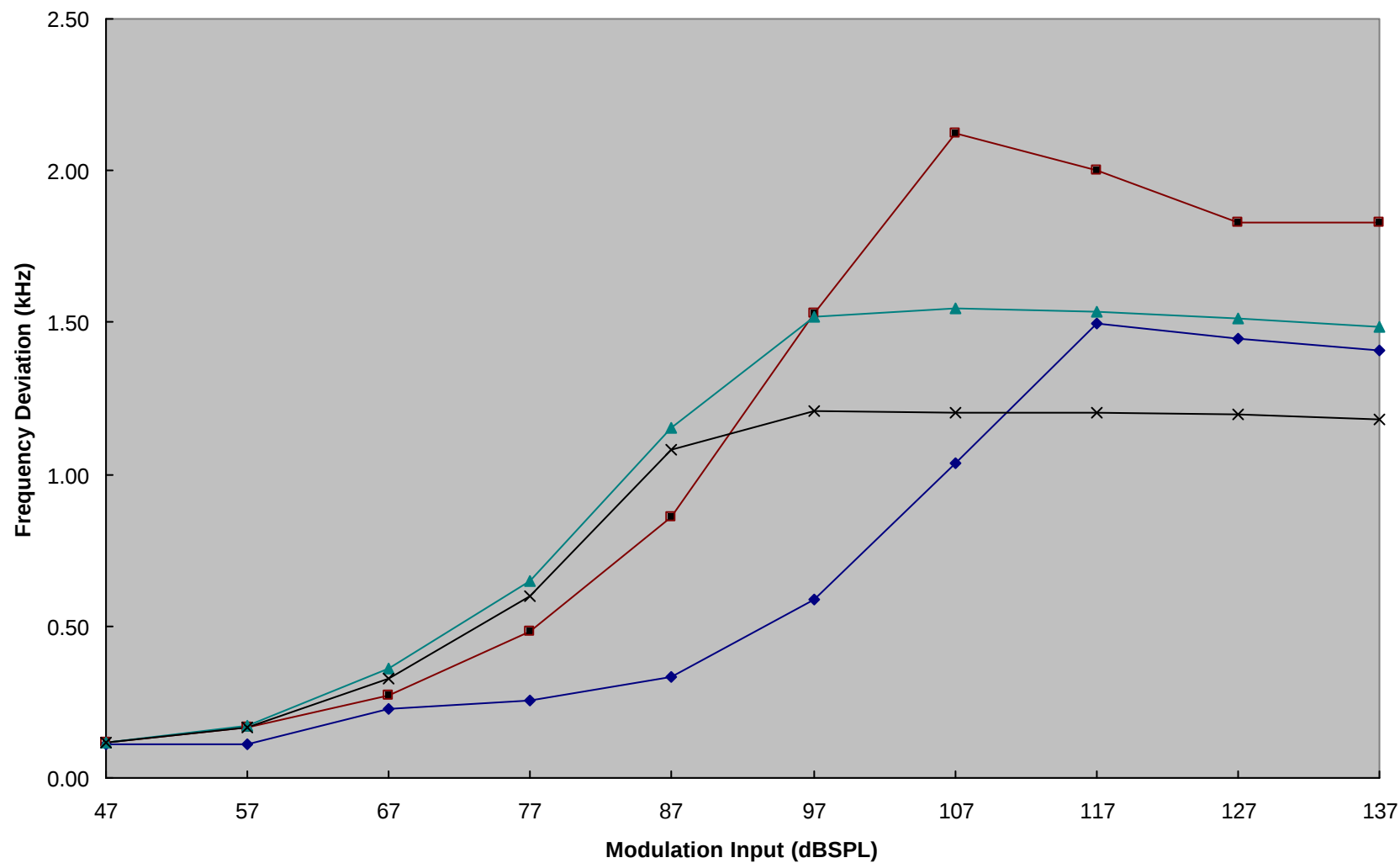
Modulation Limiting Characteristic
