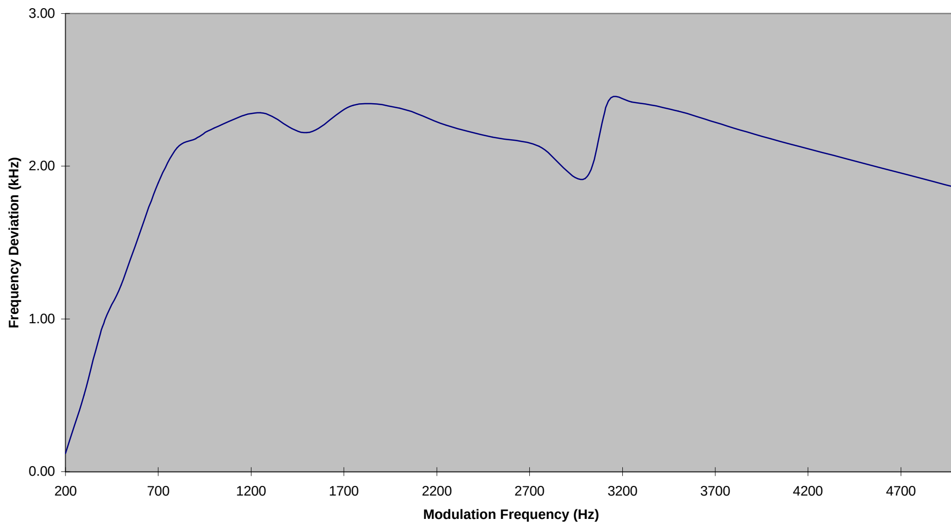
Modulation Frequency Response (Model: T5100)
