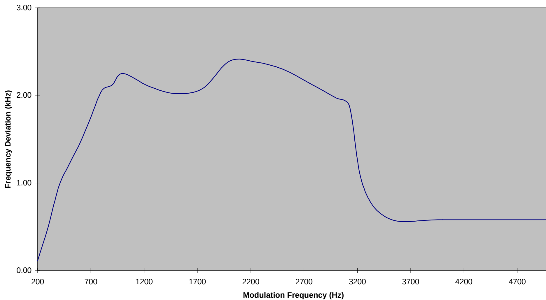
Modulation Frequency Response (Model: T5200)
