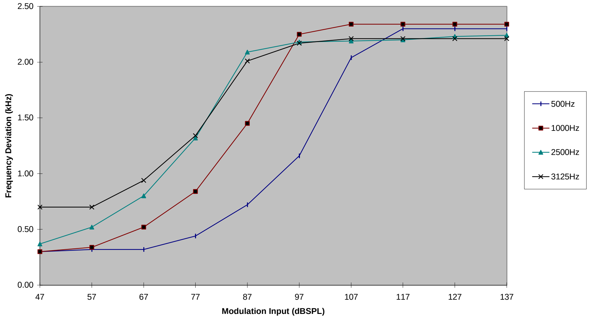
Modulation Limiting Characteristic (Model: T5100)
