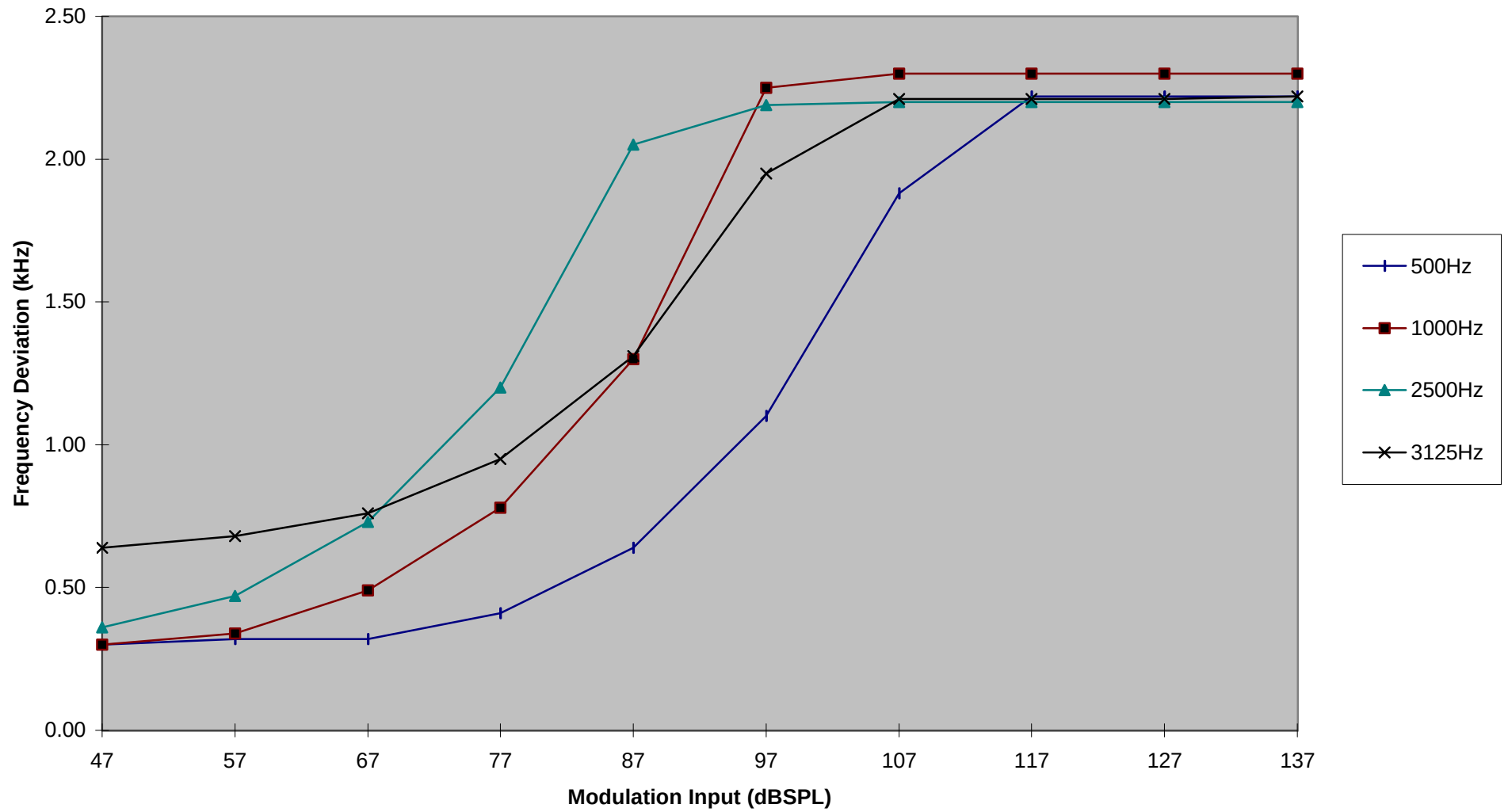
Modulation Limiting Characteristic (Model: T5200)
