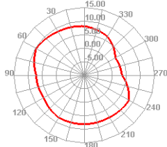
Bluetooth 78 TRP H
