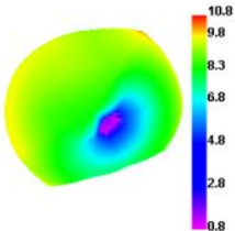
Bluetooth 78 TRP
