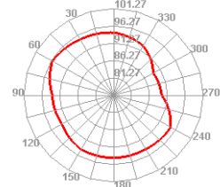
Bluetooth 78 TIS H
