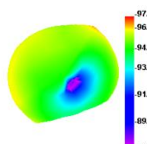
Bluetooth 78 TIS
