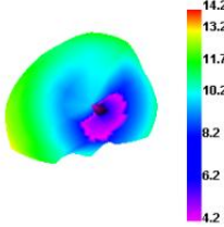
Bluetooth 0 TRP
