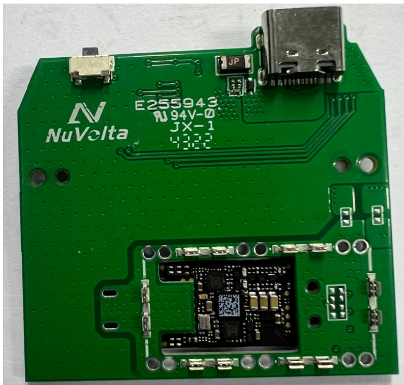
PCBA 2 – Bottom View (without shielding)
