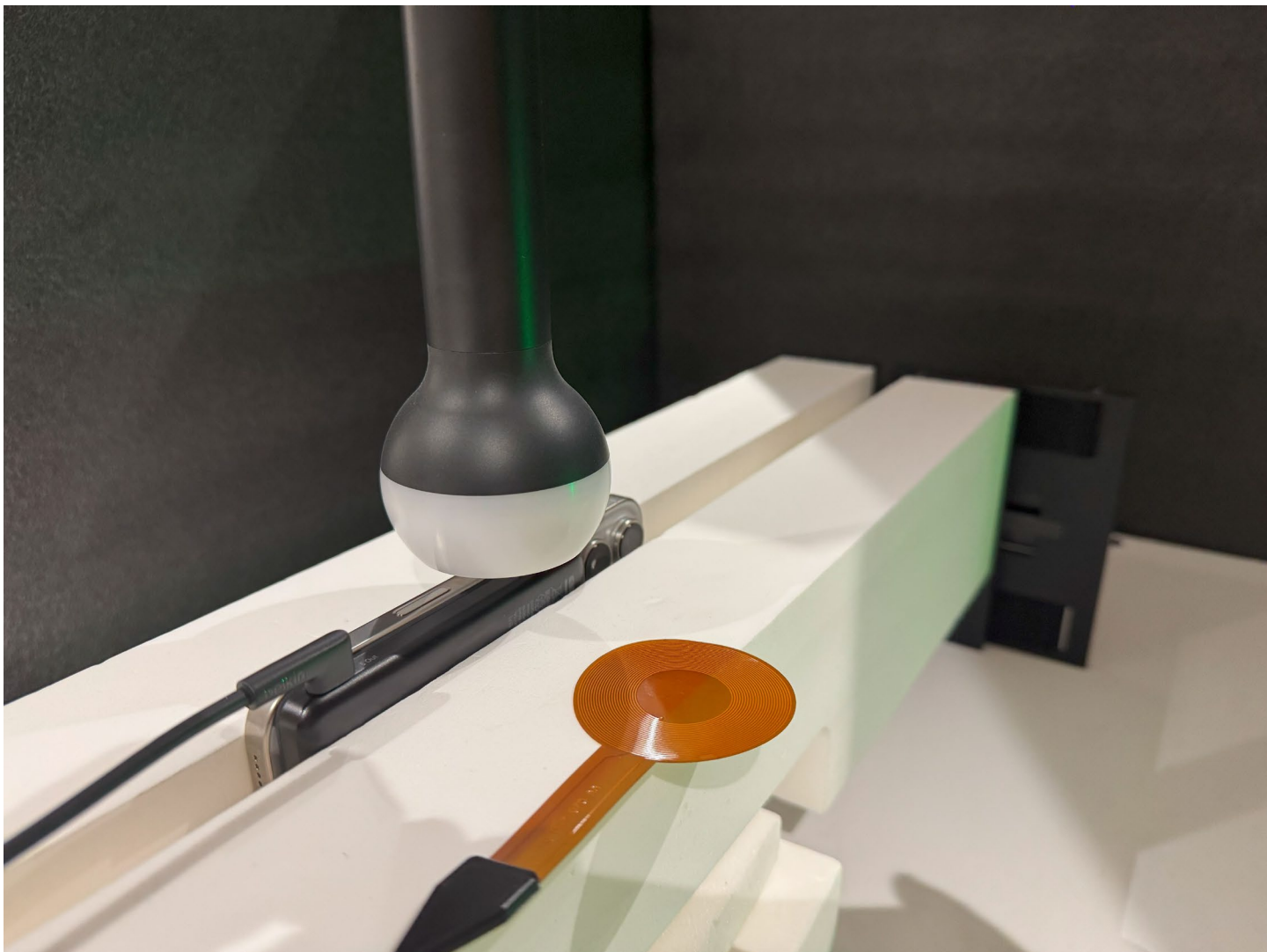
Figure F – Right Surface 0mm 111-148 kHz, Model: BPD010
