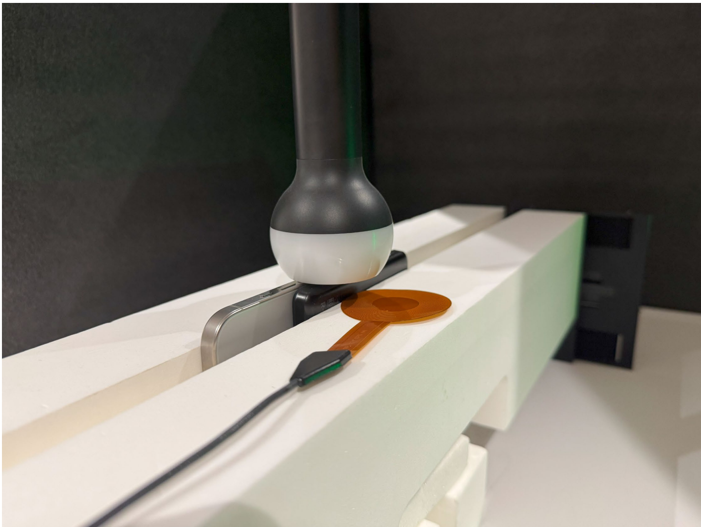
Figure E – Left Surface 0mm 111-148 kHz, Model: BPD010
