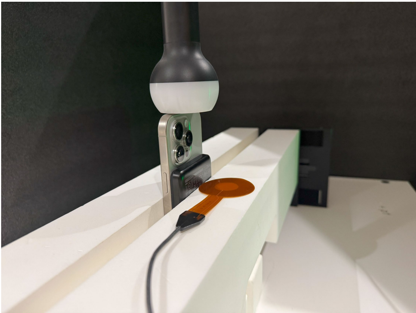
Figure C – Top Surface 0mm 111-148 kHz, Model: BPD010
