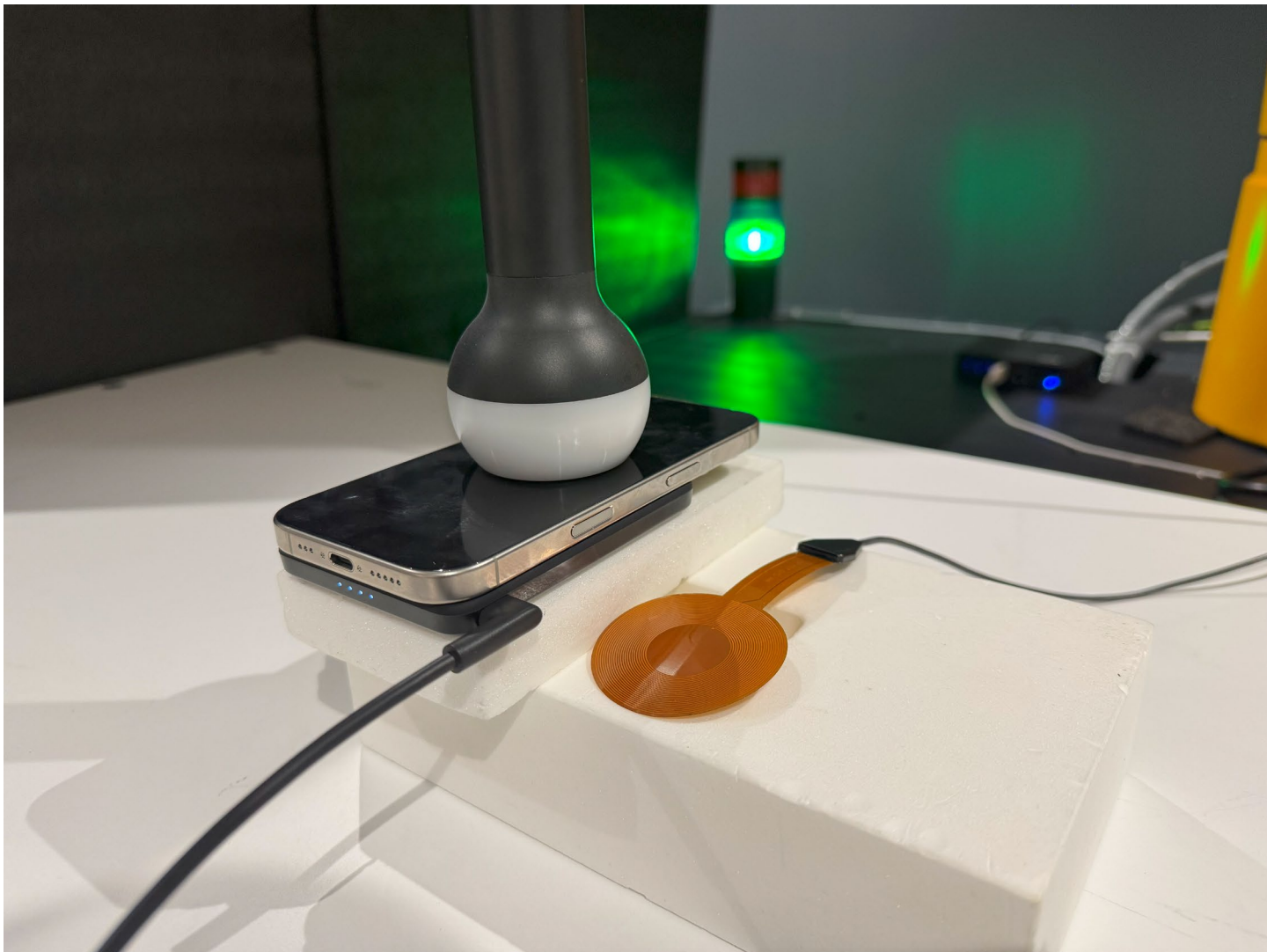
Figure A – Front Surface 0mm 111-148 kHz, Model: BPD010
