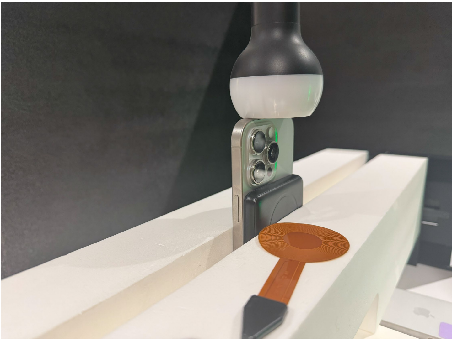
Figure I – Top Surface 0mm 111-148 kHz, Model: BBA009
