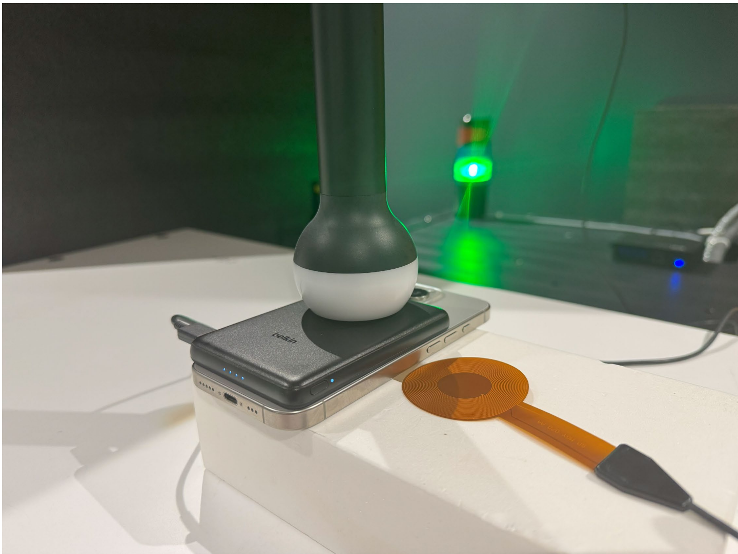
Figure H – Back Surface 0mm 111-148 kHz, Model: BBA009
