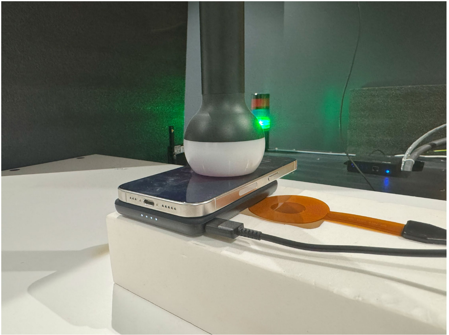
Figure G – Front Surface 0mm 111-148 kHz, Model: BBA009
