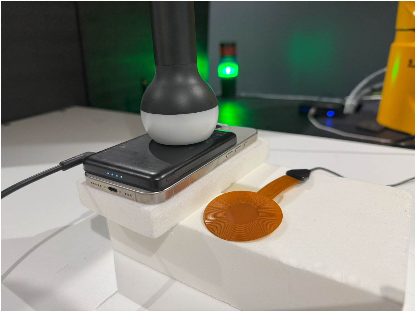
Figure B – Back Surface 0mm 111-148 kHz, Model: BPD010
