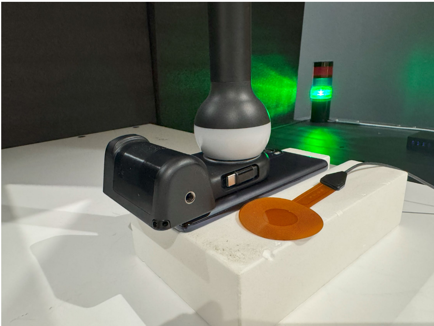
Figure B – Back Surface 0mm 111-148 kHz
