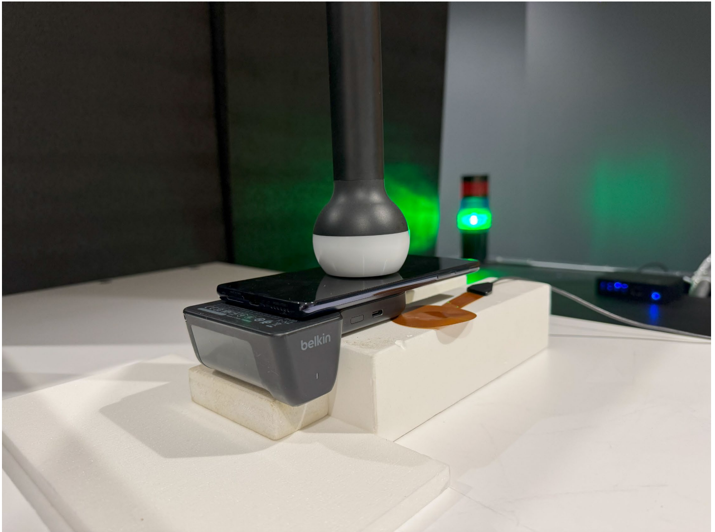
Figure A – Front Surface 0mm 111-148 kHz
