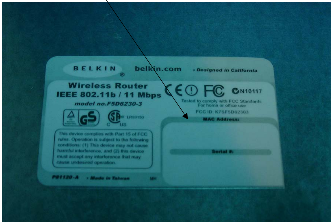
Bottom Side of EUT/Proposed FCC ID Label Location
