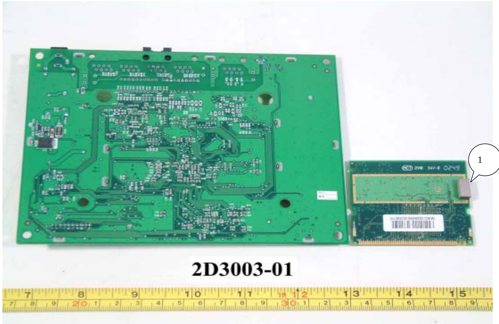
Rear side of Main Board and daughter board
