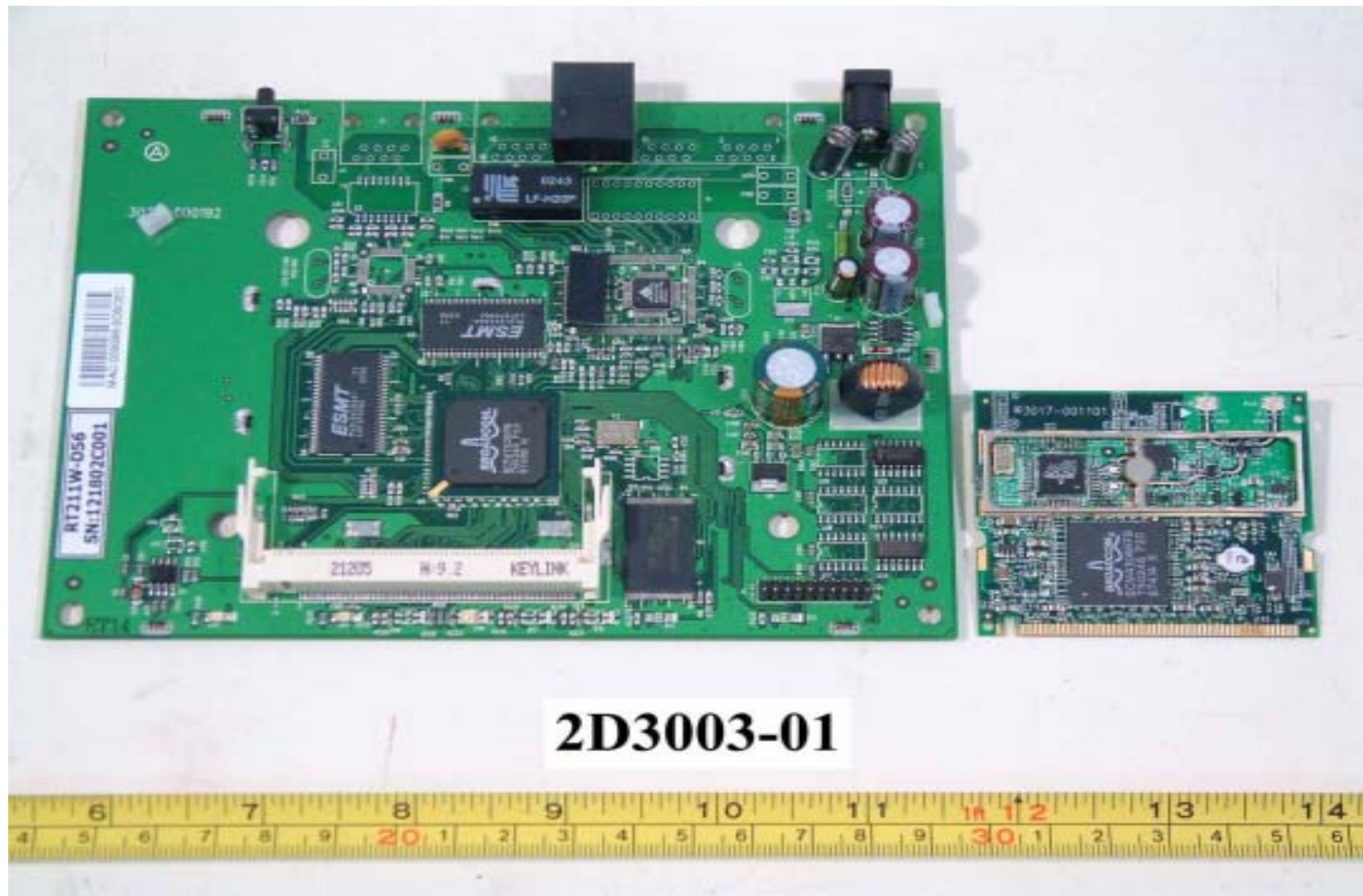
Front side of Main Board and daughter board
