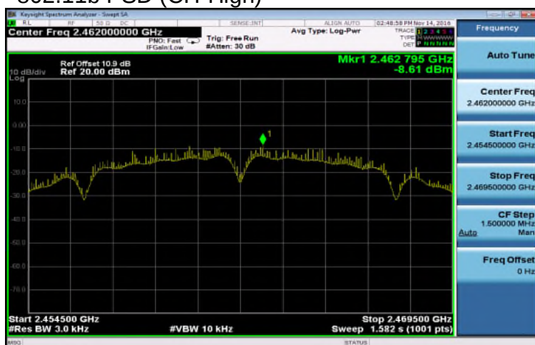
802.11b PSD (CH-High)
