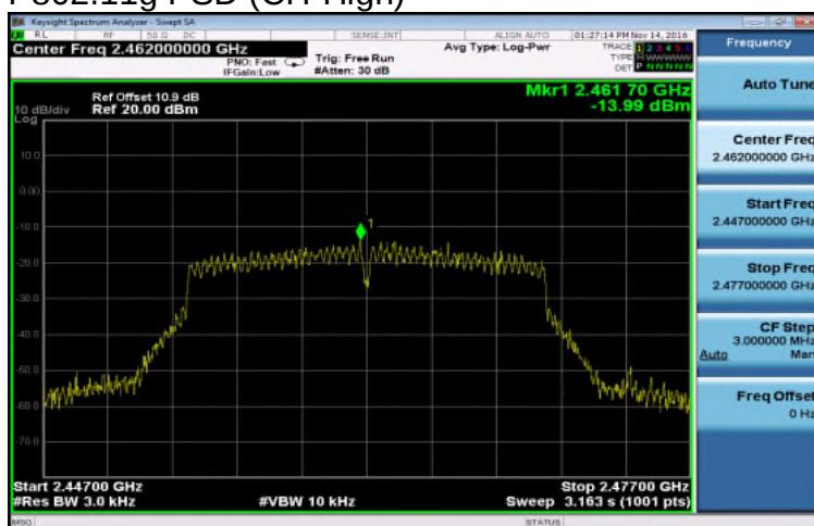
P802.11g PSD (CH-High)
