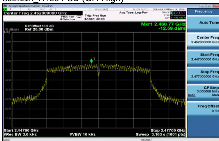
802.11n_HT20 PSD (CH-High)
