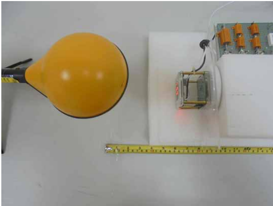
H-Field (Charging Mode with Load with 3mm gap - Z-axis)
