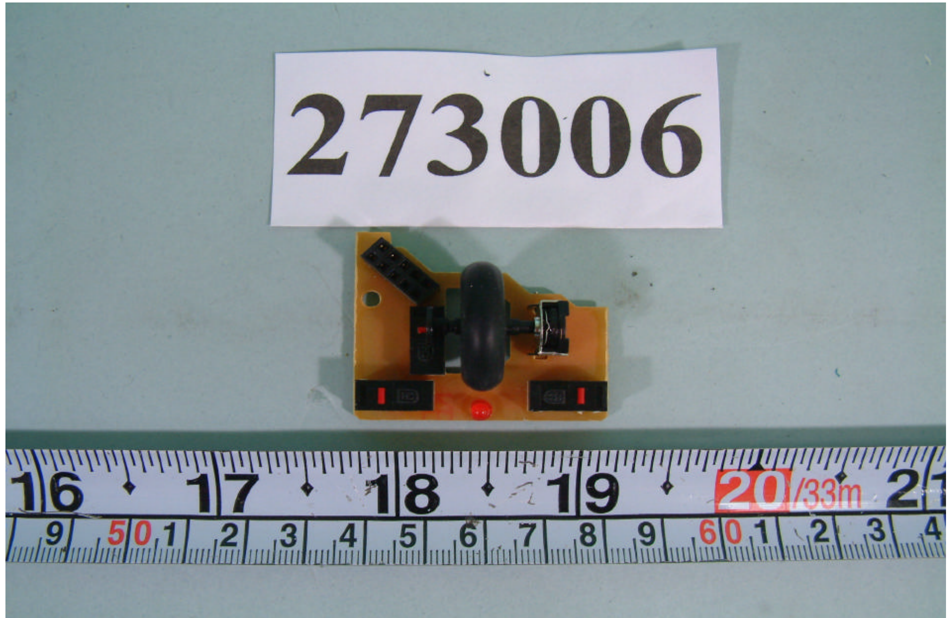
Front side of Scroll Wheel Board
