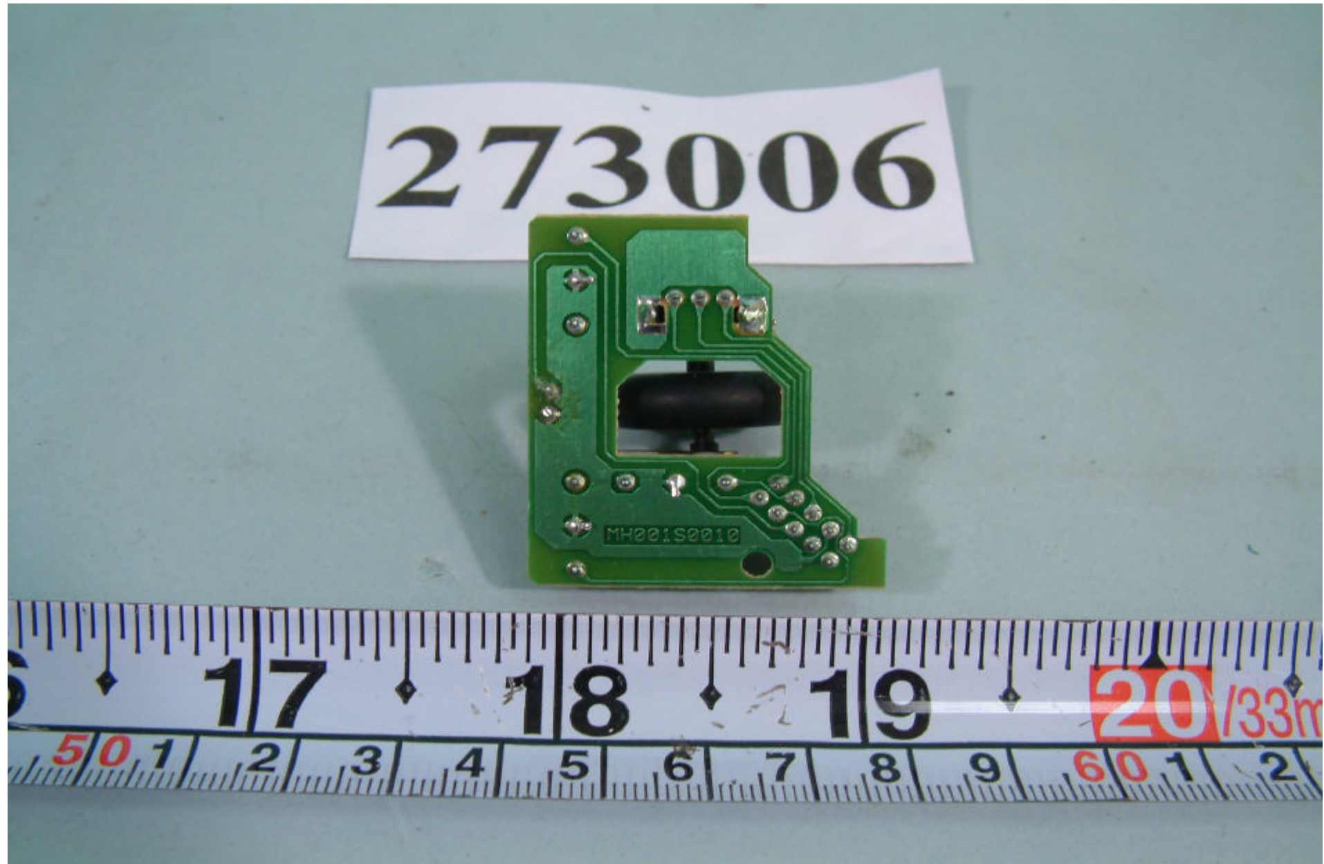
REAR side of Scroll Wheel Board
