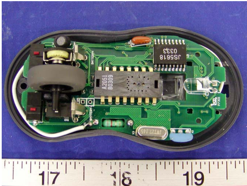
Transmitter Chassis – Cover Off View
