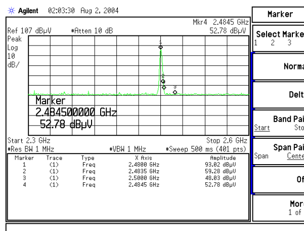
Figure Channel 78: (Vertical)
