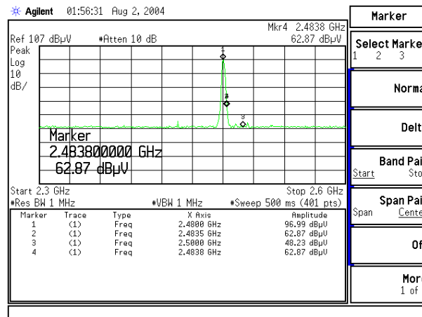
Figure Channel 78: (Vertical)
