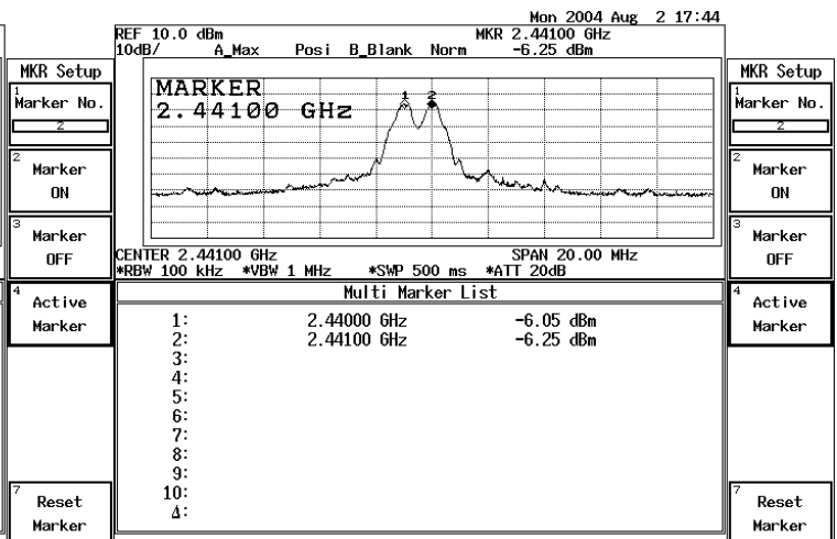
Channel 39 2441MHz
