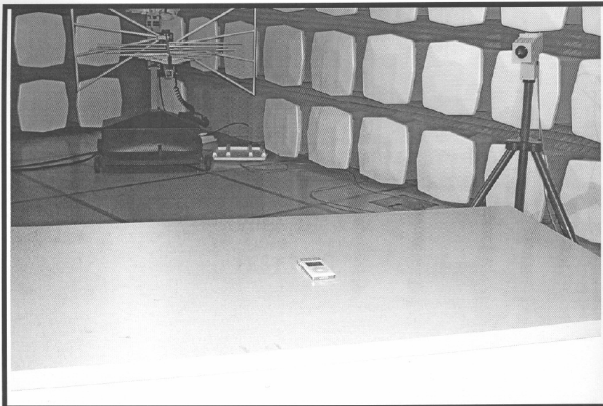
Photograph Description: Radiated set-up
