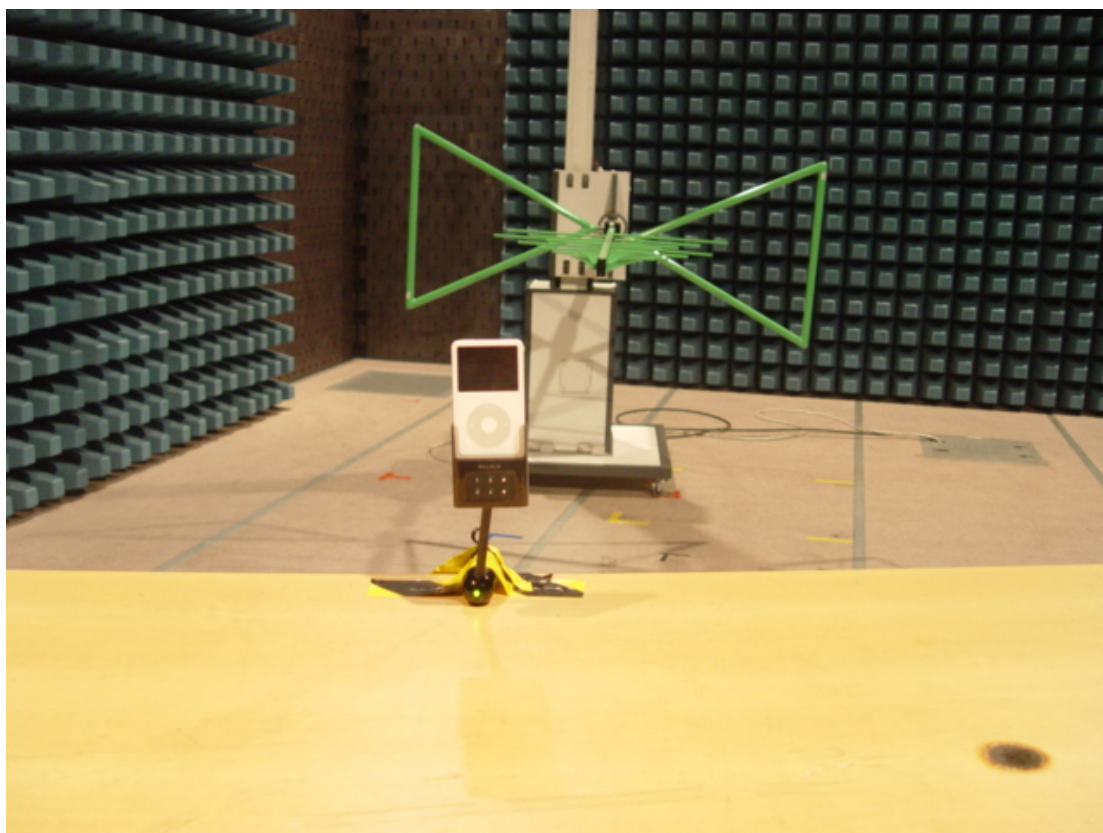
Photo 1 Radaited Emission Test
