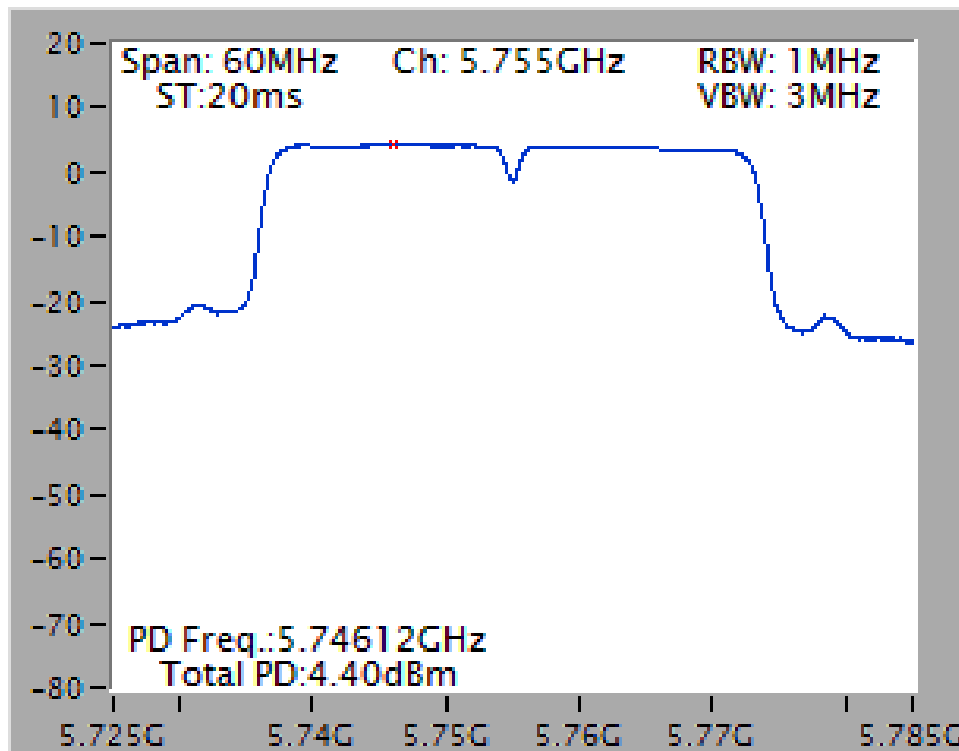
Power Density Plot on Configuration IEEE 802.11n MCS8 HT40 / Chain 1 + Chain 2 / 5755 MHz
