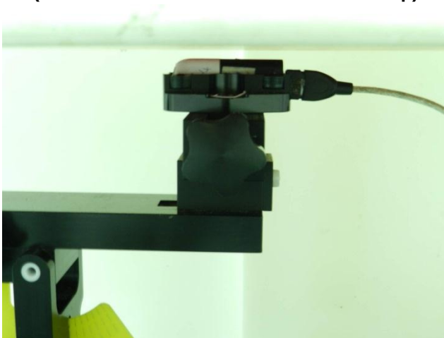
Direct Laptop Plug-in USB Configuration 4 (Vertical Back with Phantom 5 mm Gap)
