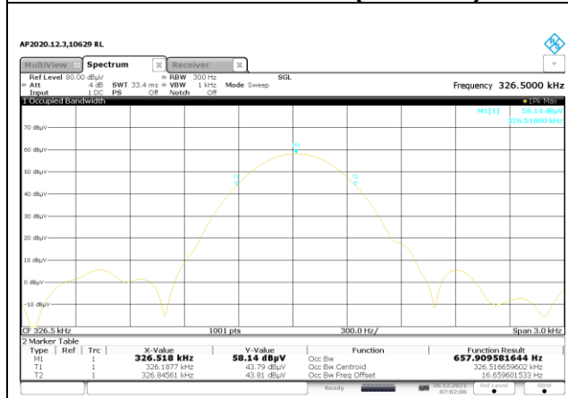
CONFIGURATION 6 (326.5kHz)
