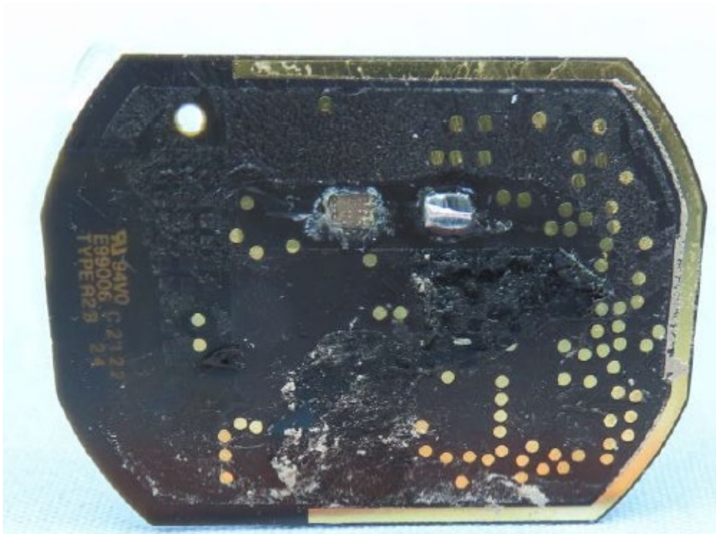
C222x PCB (MagSafe iPhones – 360 kHz) – Bottom View
