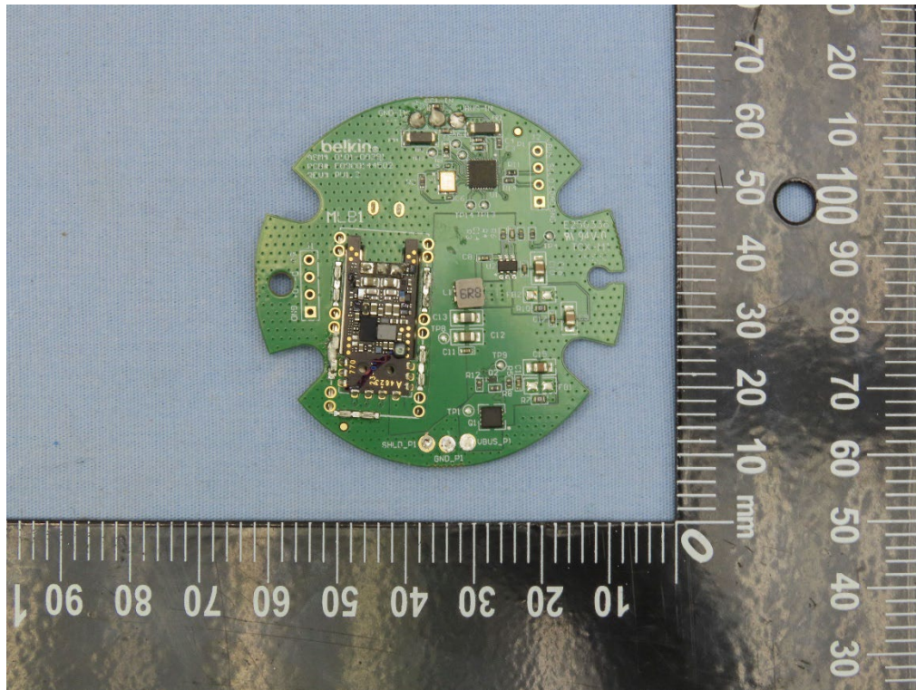
PCBA Back side (Shield Installed)
