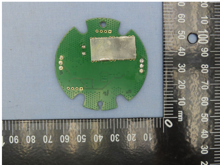
PCBA Back side (Shield Installed)
