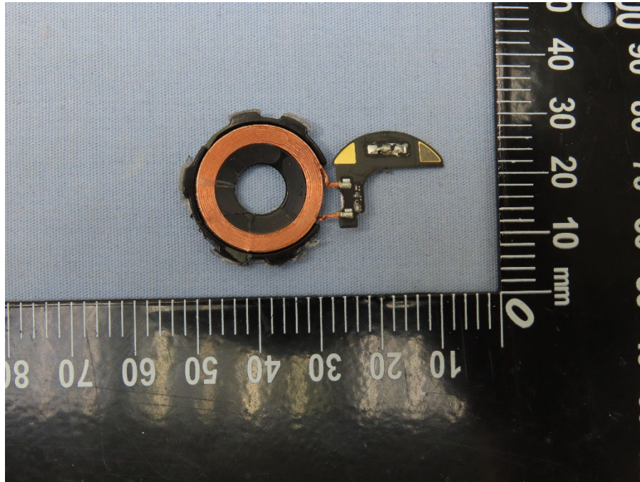
Apple Watch Coil (326.5kHz/1778kHz)
