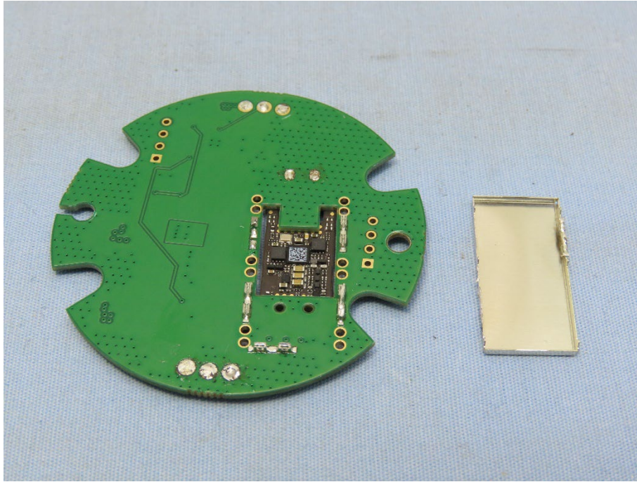
PCBA Back side (Shield Removed)
