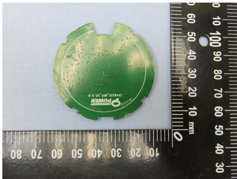
MPP Qi2 PCBA Back Side
