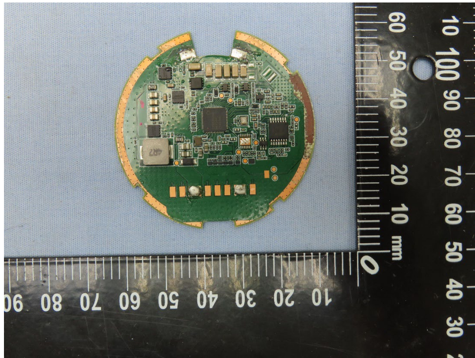
MPP Qi2 PCBA Top Side
