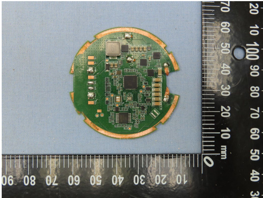
Qi2 MPP PCBA (Bottom)
