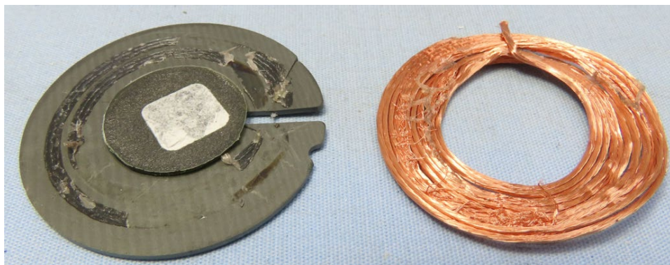
Qi2 MPP Coil (Bottom)
