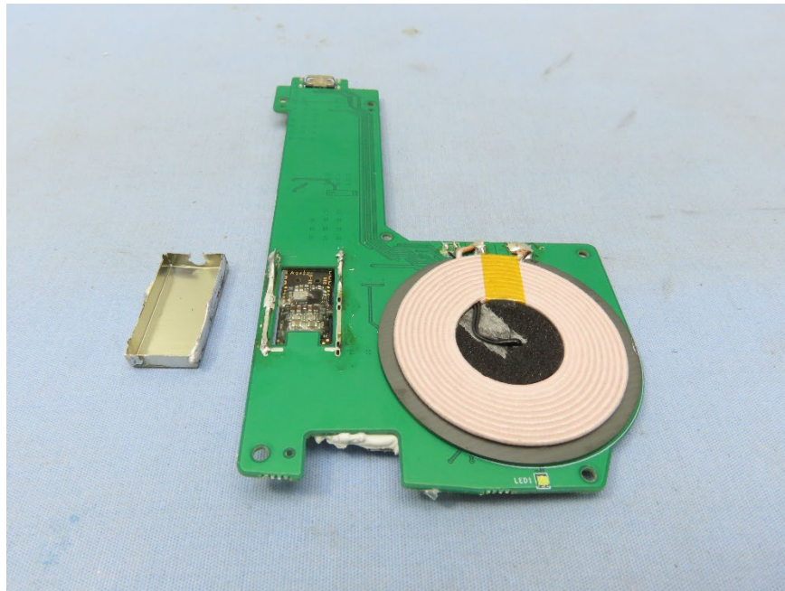
Main PCBA (Bottom) + AirPods Coil (Bottom)
