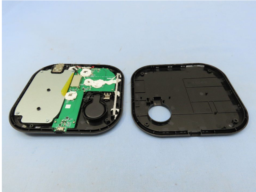
Main PCBA (Top)
