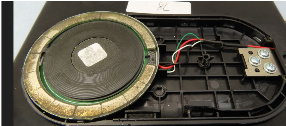
Qi2 MPP Coil (Top)
