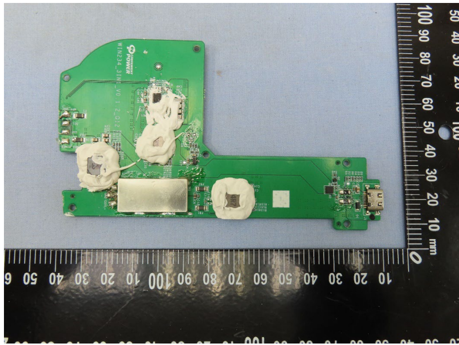
Main PCBA (Top)
