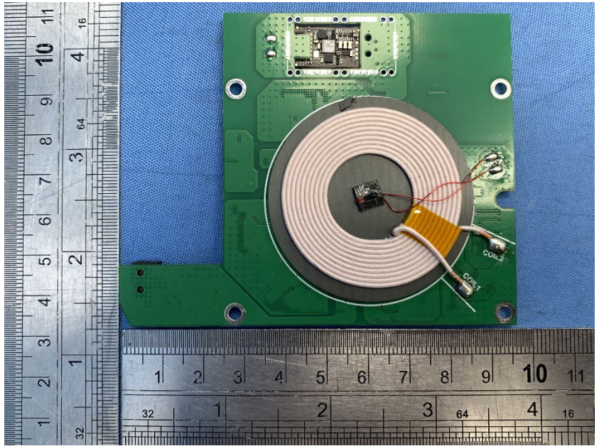
Main Board Coil and PCBA (111-148kHz)
