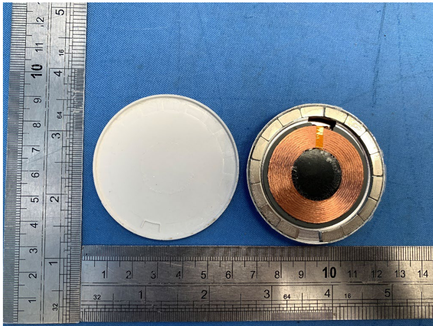
Qi2 MPP/BPP Coil and PCBA (127.7kHz, 360kHz)
