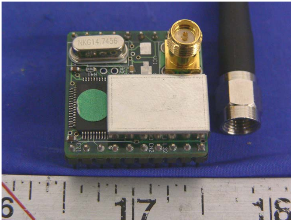
EUT – Component View with Shielding
